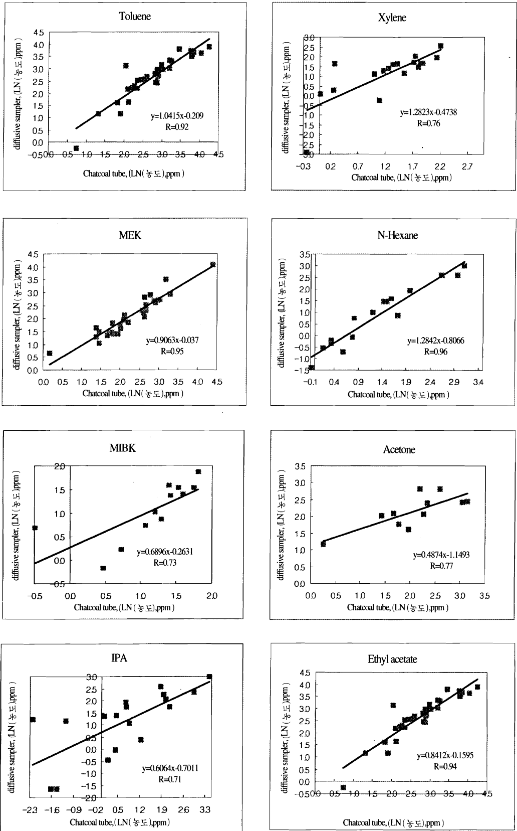
Fig. 1. Relationship between charcoal tube and a diffusive sampler method for organic solvents.
