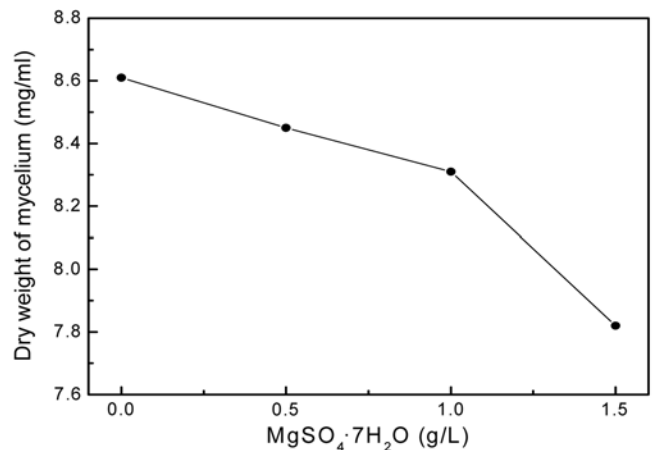
Fig. 8. Effect of MgSO_4 \cdot 7H_2O concentration on the mycelial growth of Inonotus obliquus .
