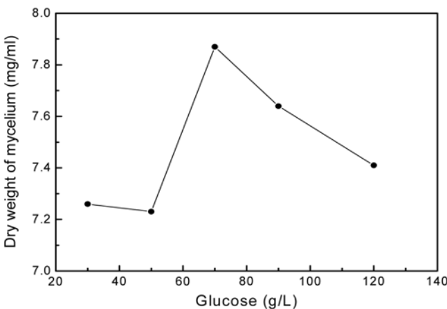
Fig. 3. Effect of glucose concentration on the mycelial growth of Inonotus obliquus .
