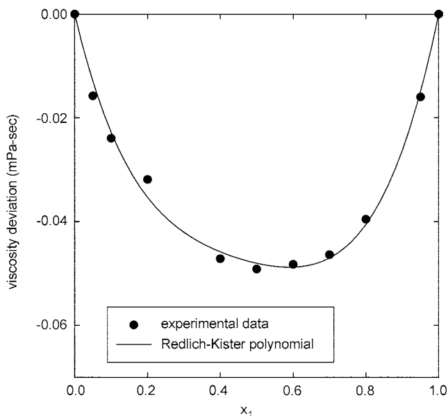
Fig. 4. Viscosity deviations for the binary system of methanol(1)+DMC(2) at 298.15 K.
