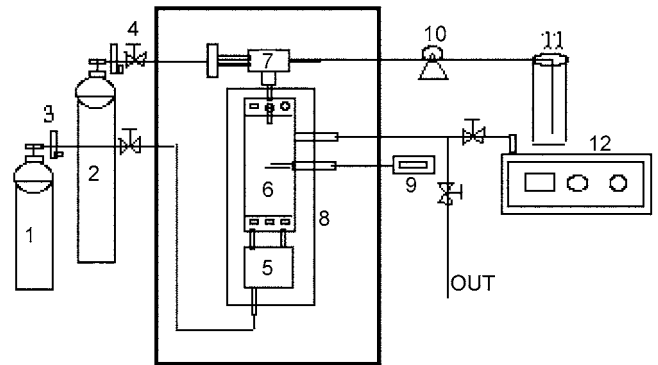
Fig. 1. Schematic diagram of SNCR proces.
