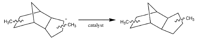
Scheme 3. Isomerization reaction of endo-THDMCPD.
