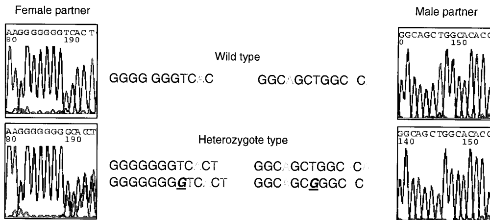
Figure 1. Identification of a mutation of a female partner (underlined G insertion) and a male partner (underlined G substitution) in exon 7 and exon 11 of the ITGB4 , respectively.
