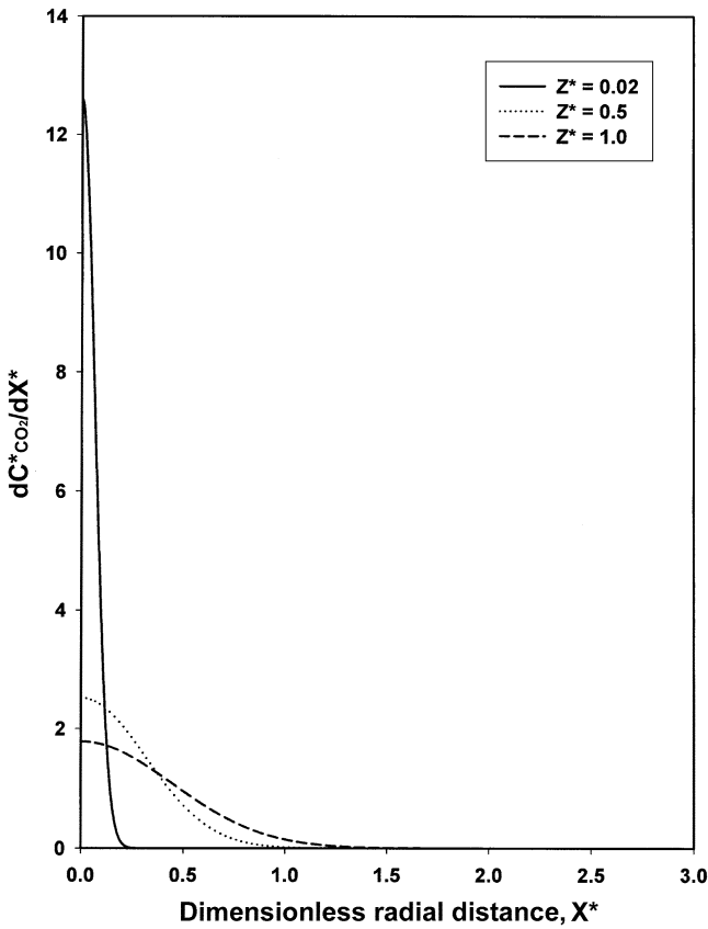
Fig. 5. Dimensionless concentration gradient of carbon dioxide in CO 2 -water system.
