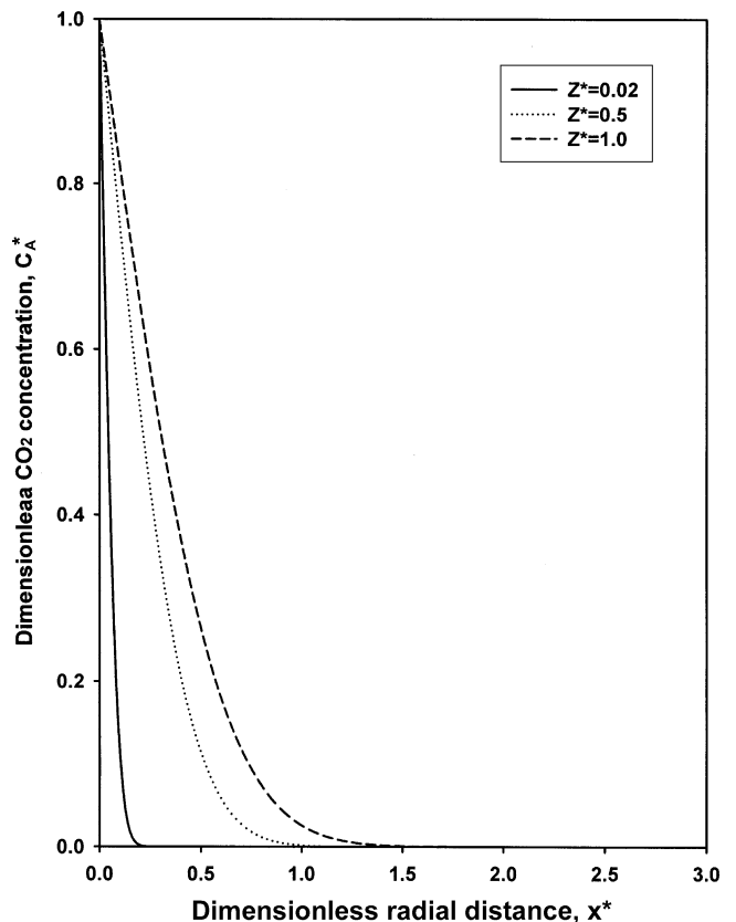
Fig. 4. Dimensionless concentration profile of carbon dioxide in CO 2 -water system.
