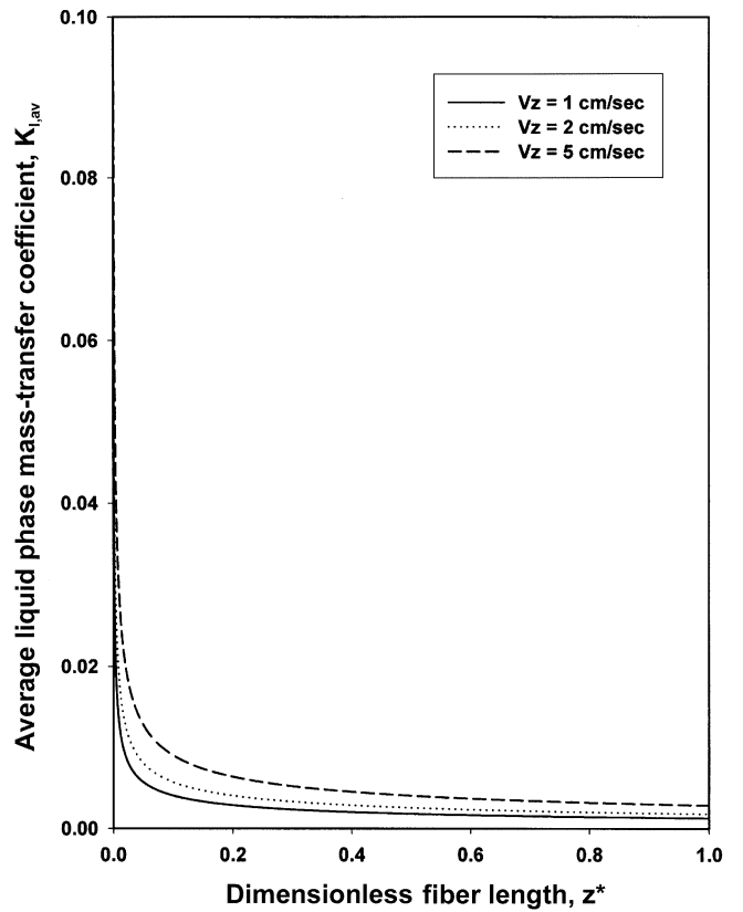
Fig. 7. The effect of absorbent flow rate on the average mass transfer coefficient in CO 2 -water system.
