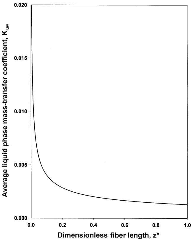
Fig. 6. Average mass transfer coefficient as a function of dimensionless fiber length in CO 2 -water system.
