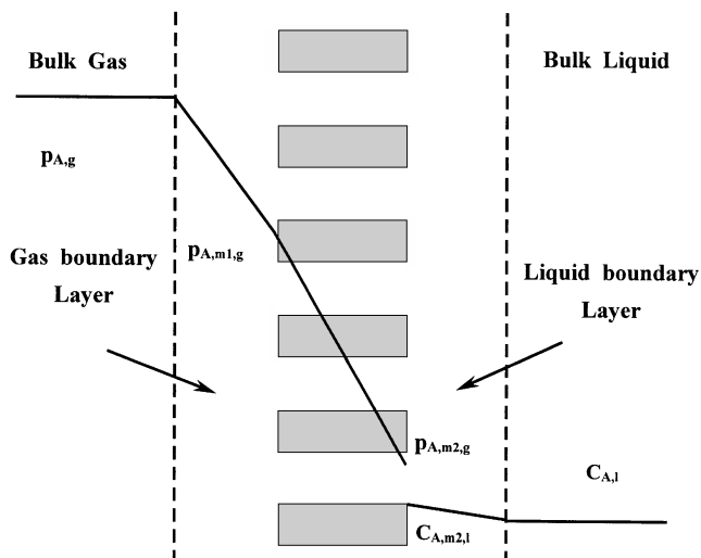
Fig. 1. Mass transfer in a porous membrane for gas absorption.
