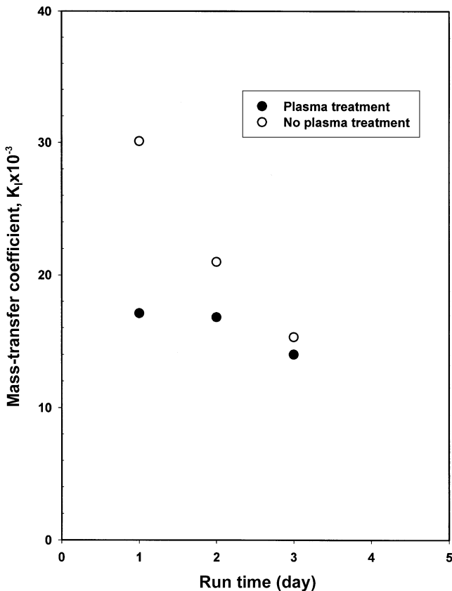
Fig. 11. The effect of plasma treatment on the mass transfer coefficient in \text{CO}_2 -MEA system.
