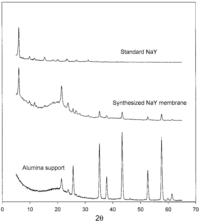
Fig. 2. XRD patterns of the NaY zeolite.
