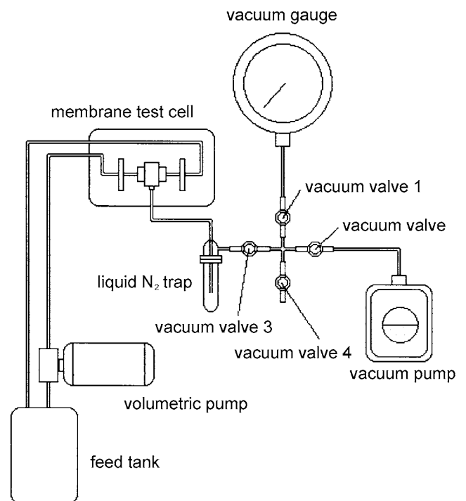
Fig. 1. A schematic of pervaporation equipment.
