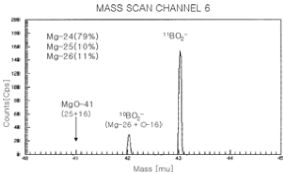
Fig. 3. The result of mass scan of BO 2 - for the boron isotope measurement.
