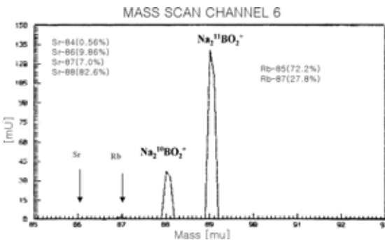
Fig. 2. The result of mass scan of \text{Na}_2\text{BO}_2^+ for the boron isotope measurement.
