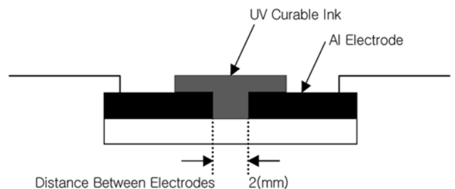
Fig. 4. Sample cell.
