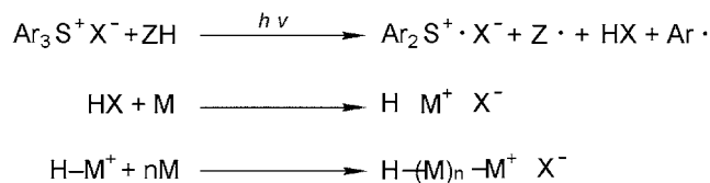
Fig. 2. Mechanism of the initiation of cationic polymerisation.
