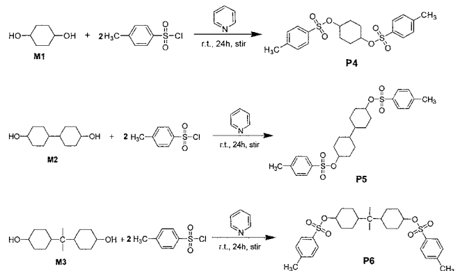
Scheme 2. Synthesis of di-type acid amplifier respectively.
