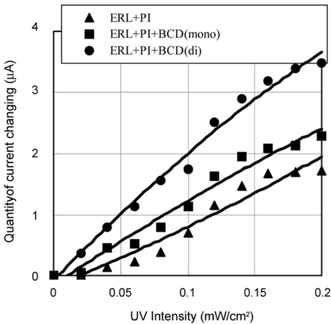
Fig. 16. Quantity of sample current changing by UV irradiation(ERL).
