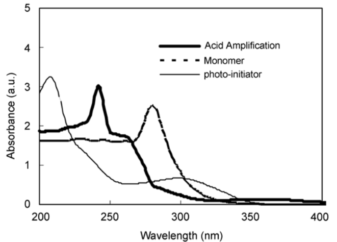
Fig. 3. Absorption spectra of compounds used in this study.
