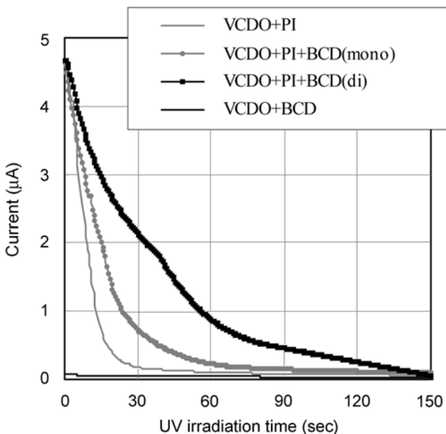
Fig. 9. Current change of P2, P5 by UV irradiation(VCDO).
