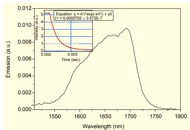
Fig. 4. Emission spectrum of the 0.02 mol% Pr 3+ doped core (Ge 30 Ga 2 Sb 8 Se 60 ) glass when pumped with an approximately 1.47 μm laser diode. The Inset figure represents both the fluorescence decay curve of the Pr 3+ : 3 F 3,4 level when monitored at 1.65 μm in wavelength, and its fitted result to the single exponential decay function (dotted line).
