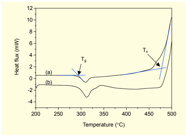
Fig. 1. Differential scanning calorimeter results of (a) the core (Ge 30 Ga 2 Sb 8 Se 60 ) and (b) clad (Ge 30 Ga 2 Sb 8 Se 55 S 5 ) glasses. The scanning rate was 10 °C/min.
