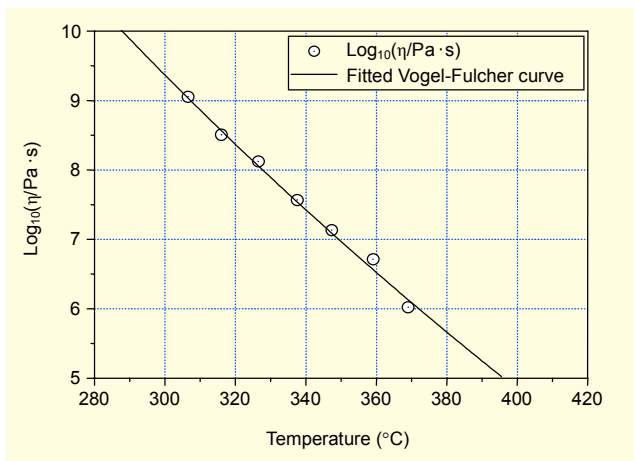
Fig. 2. Viscosity change with temperature measured by penetration viscometer method for Ge 30 Ga 2 Sb 8 Se 55 S 5 glass. A solid line represents the fitted result of the data to the Vogel-Fulcher equation.
