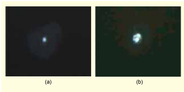
Fig. 6. Transmitted image of the 1.31 \mu\text{m} light source at the end of the fabricated selenide fiber using (a) single mode and (b) multi-mode. The image was taken from a CRT monitor connected with an IR CCD camera.
