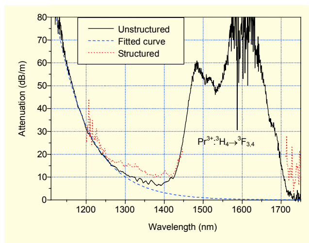
Fig. 7. Measured attenuation loss of the \text{Ge}_{30}\text{Ga}_2\text{Sb}_8\text{Se}_{60} glass fiber doped with 0.02 mol% \text{Pr}^{3+} without cladding material (solid line) and its fitted result for the background loss (dashed line). Attenuation loss measured from the multi-mode fiber is also presented (dotted line).
