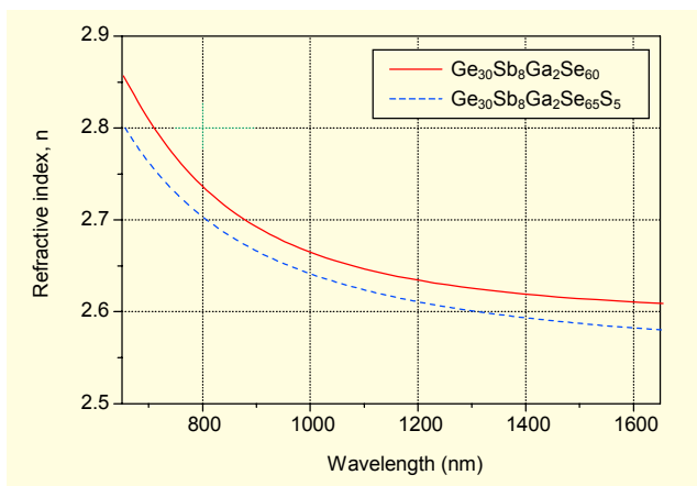
Fig. 3. Refractive index change with wavelengths of the core (solid line) and clad (dashed line) glasses.
