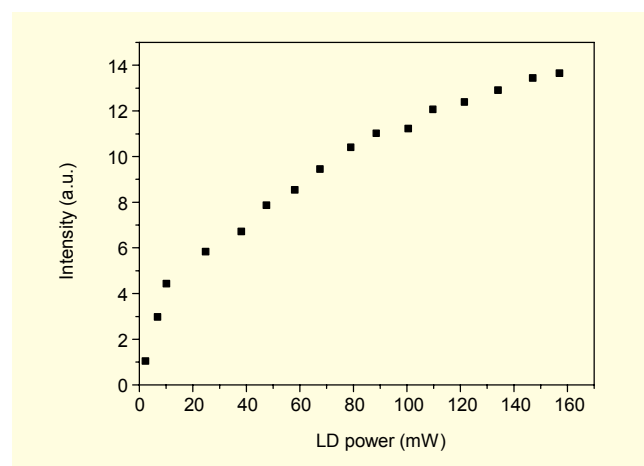
Fig. 8. Peak intensity change of the spontaneous emission varying output power of the 1.49 \mu\text{m} laser diode. Emission intensity has been monitored at 1.64 \mu\text{m} with OSA resolution of 10 nm.
