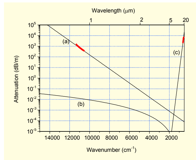
Fig. 5. Theoretically calculated attenuation loss based on the experimental results for \text{Ge}_{30}\text{Ga}_2\text{Sb}_8\text{Se}_{60} glass considering (a) electronic transition, (b) Rayleigh scattering, and (c) multiphonon absorption within the glass.
