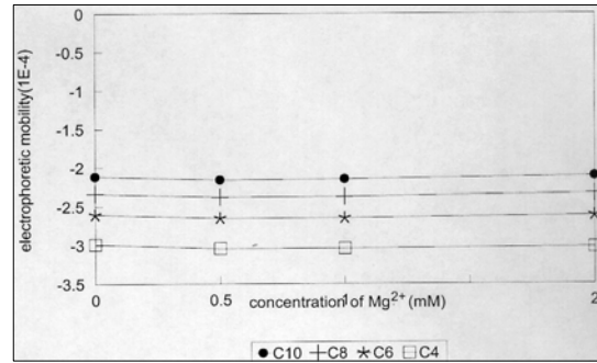
Fig. 5. Electrophoretic mobilities of short chain carboxylates in various Mg^{2+} concentration.
