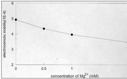
Fig. 4. Variation of the electroosmotic mobility in various Mg^{2+} concentration.
