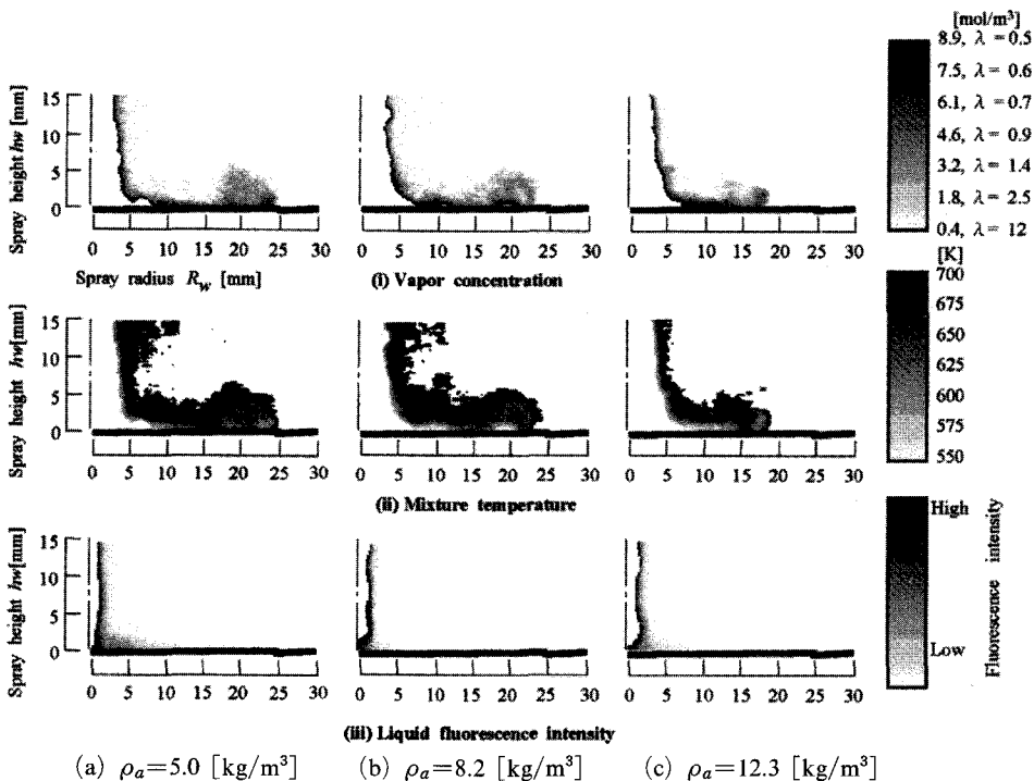
Fig. 4 Temporal change in impinging spray image with exciplex fluorescence method at t=1.10 [ms] from injection start ( p_{inj}=72 [MPa] Q_{inj}=12.0 [mg] T_w=550 [K] Z_w=40 [mm])
