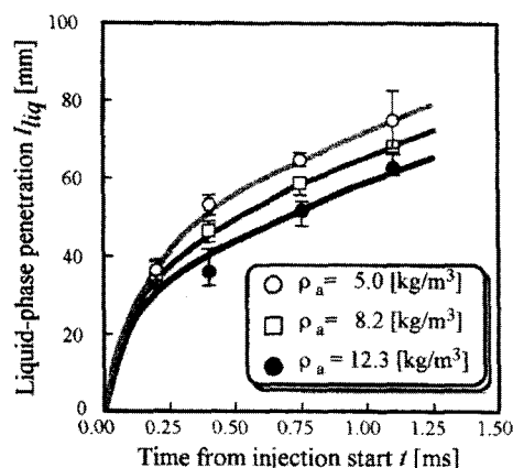
(b) Liquid-phase penetration I_{liq}
