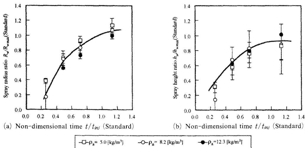
Fig. 5 Temporal change in spray radius R_w and height h_w ( p_{inj}=72 \text{ [MPa]} Q_{inj}=12.0 \text{ [mg]} T_w=550 \text{ [K]} Z_w=40 \text{ [mm]} )
