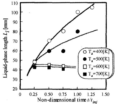
Fig. 11 Liquid-phase length ( L_l ) variation for ambient temperature change
