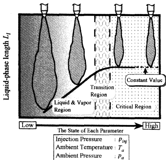
Fig. 12 History of liquid-phase length for each of the experiment conditions in diesel spray
