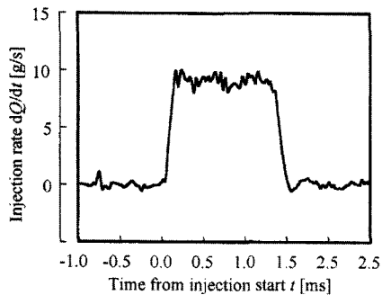
Fig. 1 Temporal change in fuel injection rate at p_{inj}=72 [MPa]
