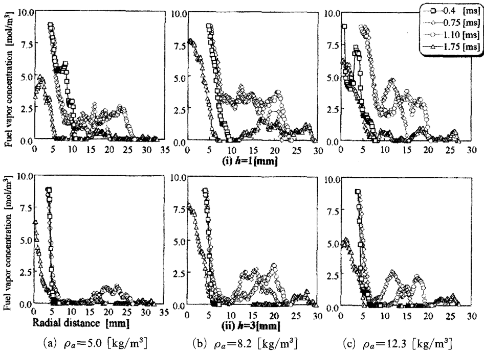
Fig. 6 Radial distribution of fuel vapor concentration ( p_{inj}=72 [MPa], Z_w=40 [mm])
