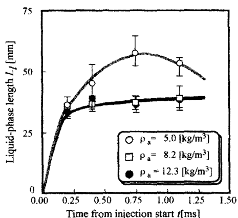
Fig. 9 Temporal change in liquid-phase length
