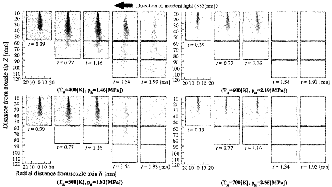
Fig. 10 Liquid-phase images with exciplex fluorescence method using 35 mm still camera ( p_{vi}=72 [MPa] Q_{vi}=12.0 [mg] \rho_a=12.3 [Kg/m 3 ])
