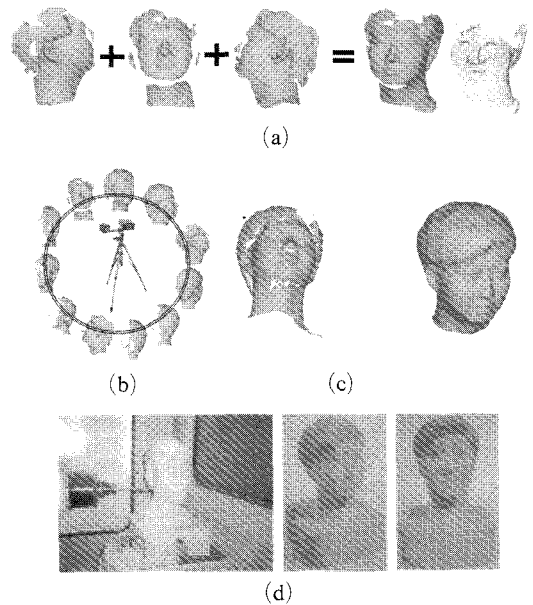
Fig. 9 Example of full 3D reverse engineering process. (a) Three individual views and their roughly aligned result; (b) eleven individual views and their roughly aligned result using extracted feature information; (c) Final model after applying hole-filling, smoothing, remeshing processes, etc.; (d) 4-axis NC machining and a physical replica (bust sculpture)
