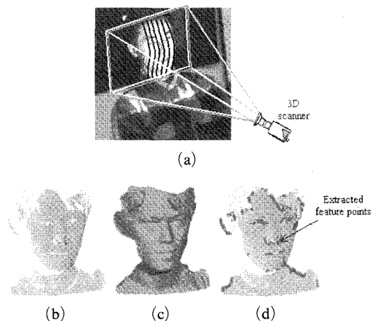
Fig. 8 The process of the reverse engineering system. (a) Projected light pattern ; (b) scanned point cloud ; (c) shaded image of created triangles ; (d) extracted features
