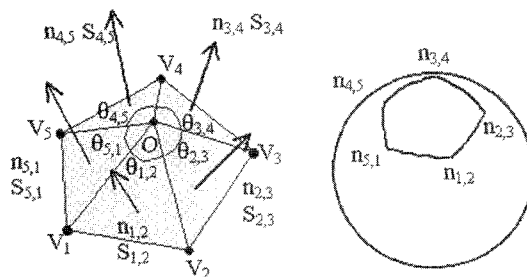
Fig. 6 The angle deficit of the polyhedron (Calladine, 1986)
