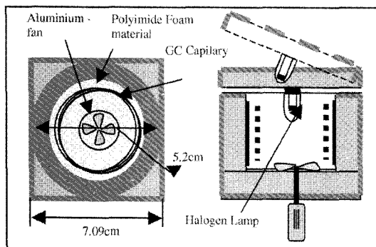
Fig. 2 Main parts of the GC oven
