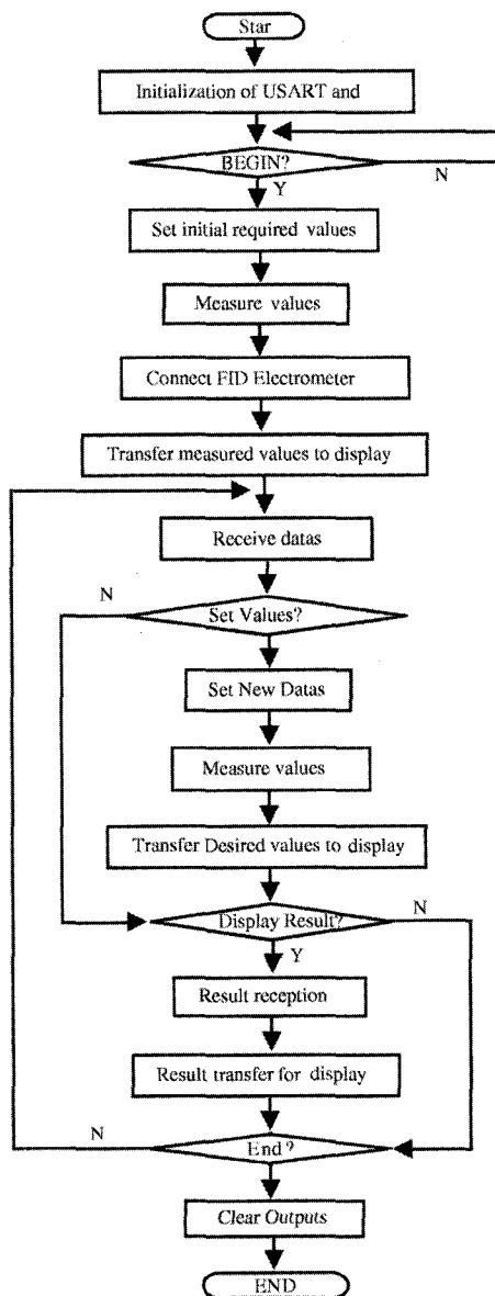
Fig. 9 Program flow diagram for the Microcontroller
