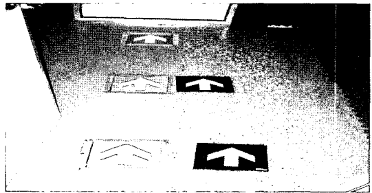
Fig. 4. Photoluminescent exit sign on the outlet floor in experimental apparatus.
