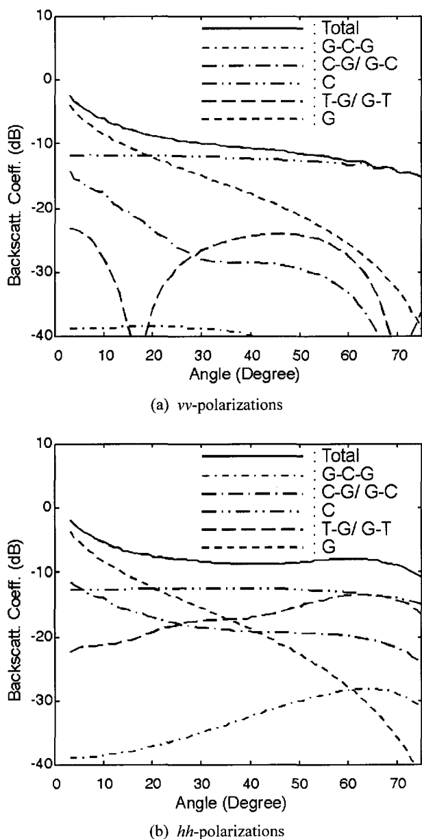
Fig. 2. Computation results for a typical forest at 5.3 GHz.
