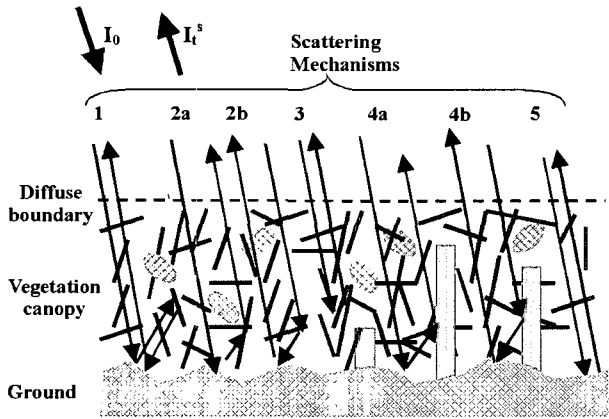
Fig. 1. Scattering mechanisms.
