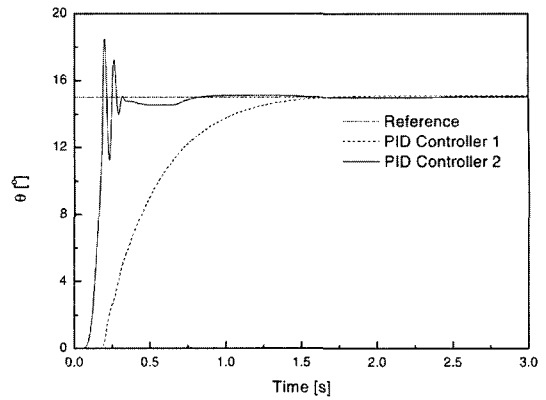
Fig. 11 Comparison between PID controller 1 and PID controller 2
