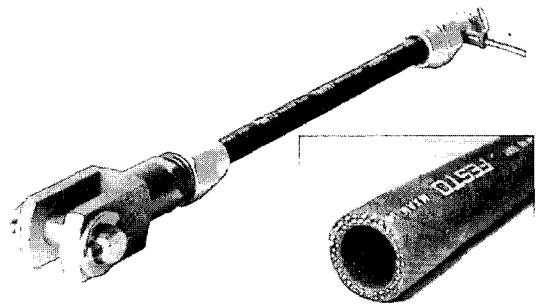
Fig. 2 Structure of the pneumatic artificial muscle
