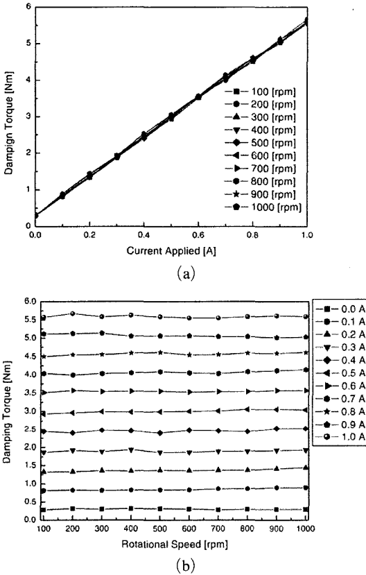
Fig. 8 Characteristics of MRB
