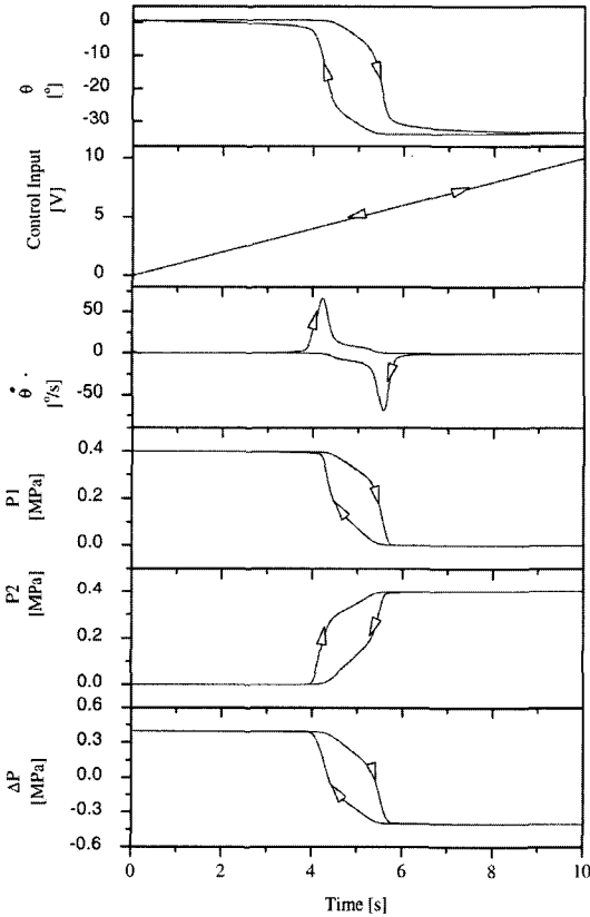
Fig. 5 Characteristics of pneumatic artificial muscle manipulator
