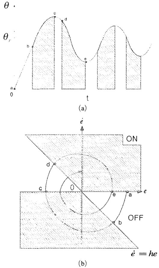
Fig. 10 Concept of phase plane switching control
