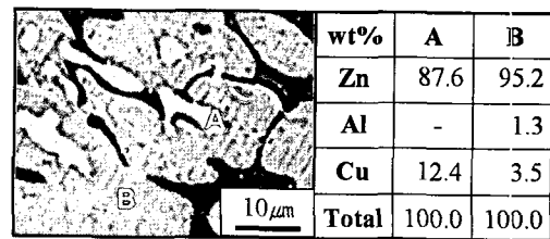
Fig. 8 Results of EPMA analysis
