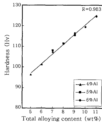
Fig. 13 Effect of total alloying content on the vickers hardness
