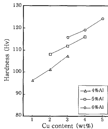
Fig. 12 Result of Vickers hardness test
