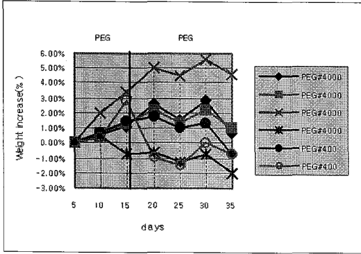
Fig.10. Weight changes in sample during the treatment impregnation with PEG#400 & PEG#4000 sol. Vacuum.
