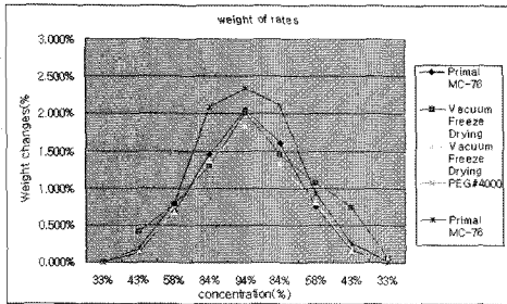
Fig. 12. Weight changes of treated samples stored in humidity-controlled chamber(sample 1, 6 treated after Primal MC-76, sample 5 treated after PEG#4000 sol, sample 2, 4 treated after Vacuum freeze drying.).
