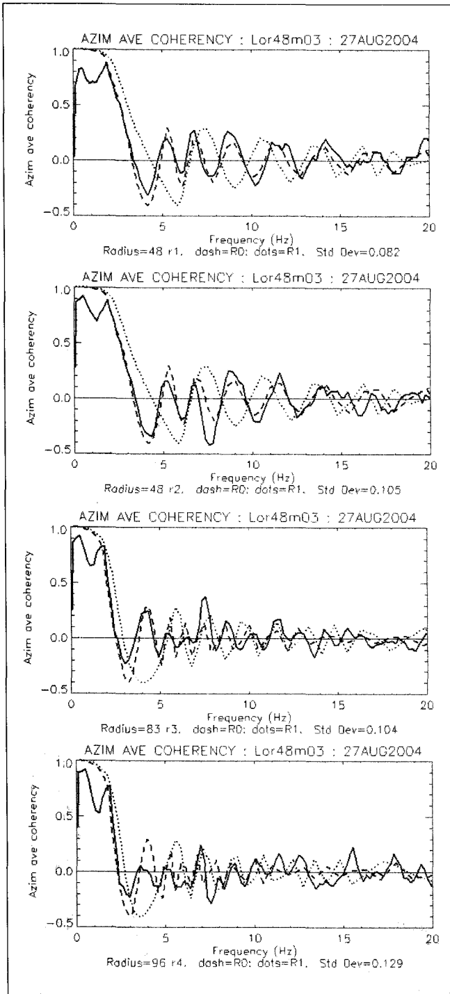
Fig. 4. Results of iterative interpretation procedure for Lorimer Street 48 m radius array. Station separations are (a) 48 m, (b) 48 m, (c) 83 m, (d) 96 m. Line types as for Figure 3.
