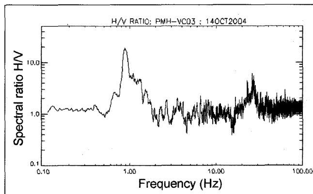
Fig. 7. Sample H/V spectral ratio. Note the distinct peak at a frequency of approximately 0.9 Hz. Similar records (at locations shown in Figure 1) were used to construct the contour map shown in Figure 8.
