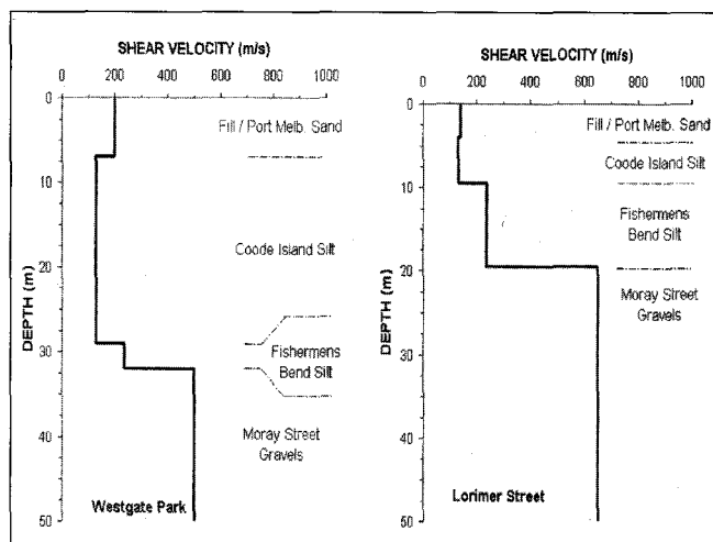
Fig. 6. Best-fit shear-wave velocity profiles corresponding to the interpreted coherency spectra shown in Figures 3 and 4 (Lorimer Street) and Figure 5 (Westgate Park).
