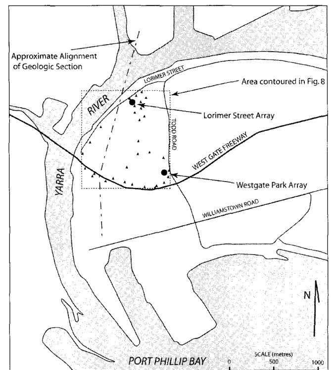
Fig. 1. Site location map indicating survey locations, proximity to major roads, and the position of the geological section shown in Fig 2. SPAC array locations are as indicated. The small triangles represent locations of single-station, 3-component recordings for H/V spectral ratios.
