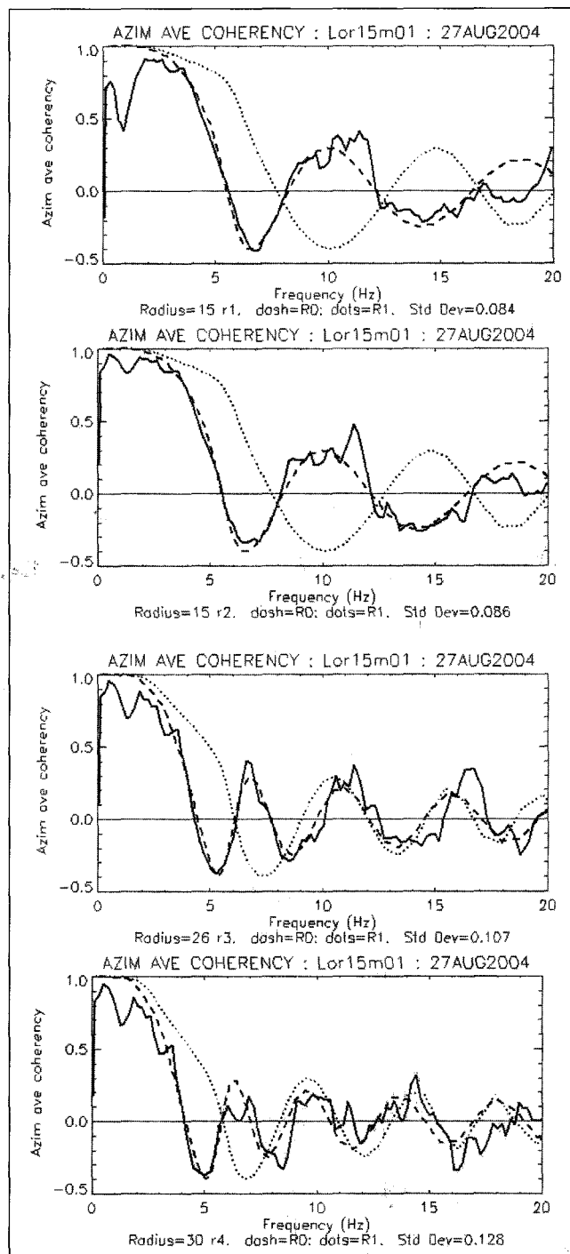
Fig. 3. Results of iterative interpretation procedure for Lorimer Street 15 m radius array. Station separations are (a) 15 m, (b) 15 m, (c) 26 m, (d) 30 m. Solid black line: field data SPAC spectrum; Dashed line: model SPAC for the layered earth shown in Figure 6, fundamental Rayleigh mode, used for iterative fitting to field data; Dotted line: model SPAC for the first higher Rayleigh mode; shown for reference purposes only since higher modes appear to be absent in this sample of field data.
