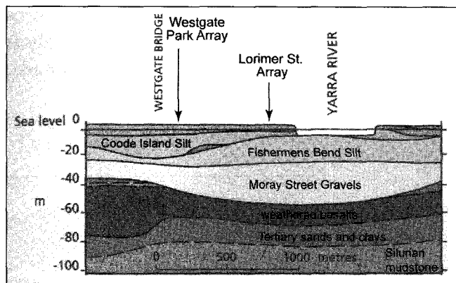
Fig. 2. Geological section through Port Melbourne and Fishermans Bend. (Reproduced from Cupper et al. (2003), Figure 11.19).
