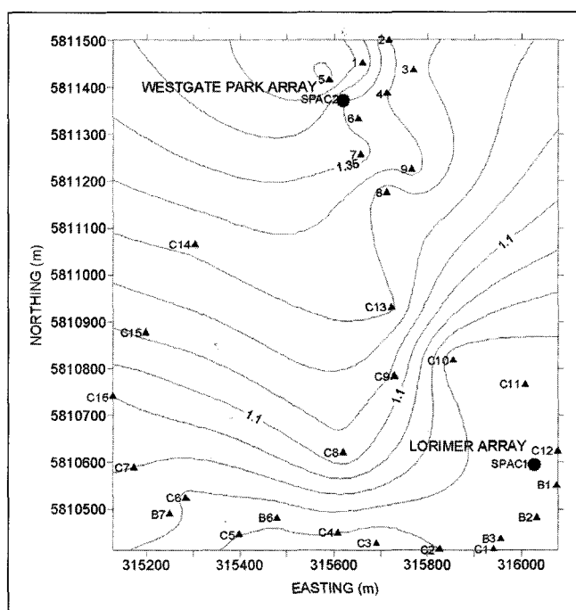
Fig. 8. Contour map showing trends in H/V spectral ratio (HSVR) peaks (in Hz), based on three-component ground motion recordings. Higher values correspond to zones where silt is thinner, firmer, or both. Triangles with station labels show site positions for HSVR data. Circles show position of arrays used for SPAC analysis. Contour interval is 0.05 Hz.
