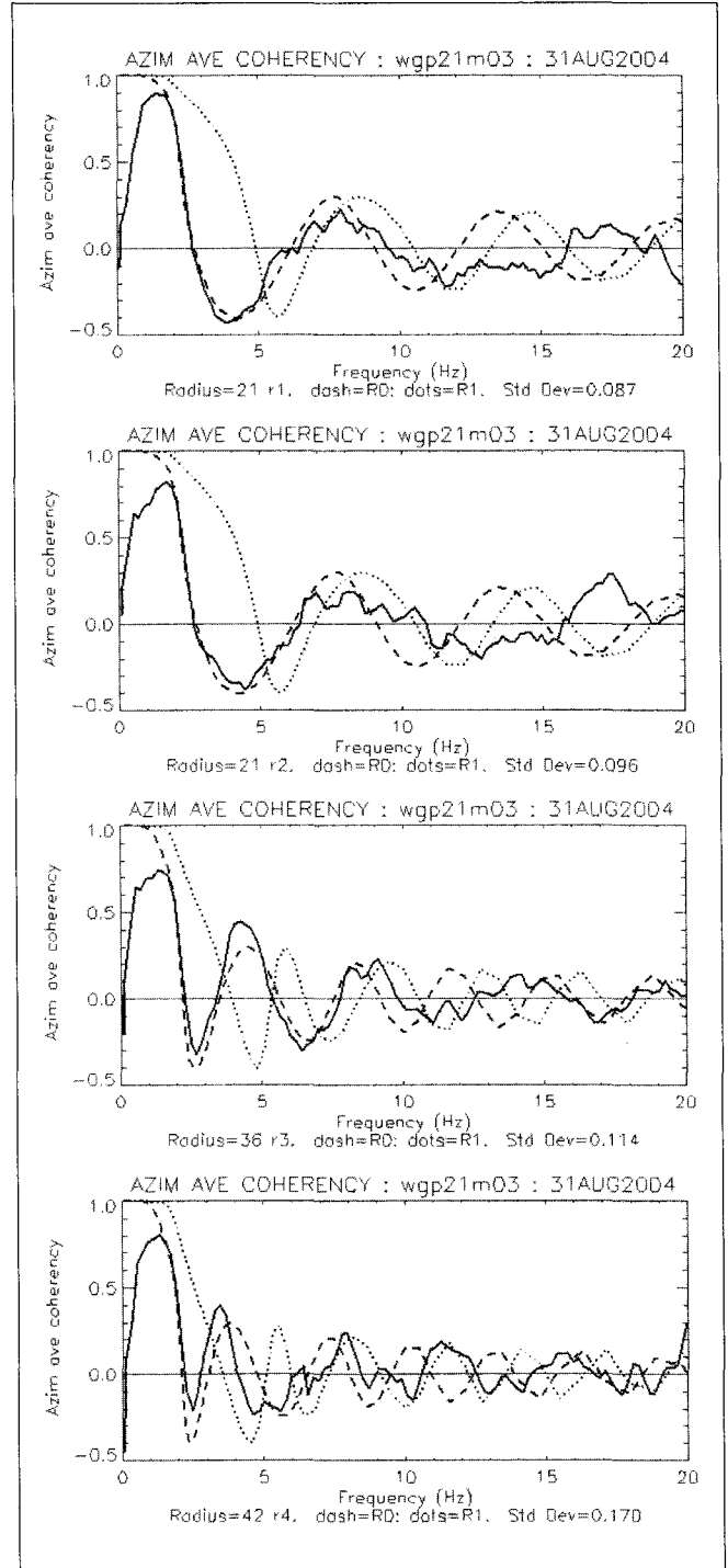
Fig. 5. Results of iterative interpretation procedure for Westgate Park 21 m radius array. Station separations are (a) 21 m, (b) 21 m, (c) 36 m, (d) 42 m. Line types as for Figure 3.
