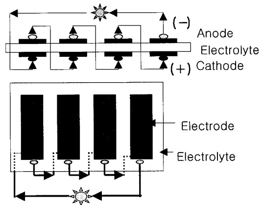
(b) Monopolar stack
