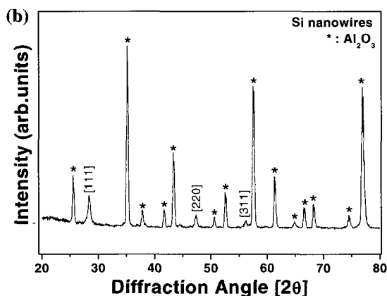
Fig. 1. (a) SEM image and (b) X-ray diffraction spectra of the Si nanowires synthesized by thermal CVD.
