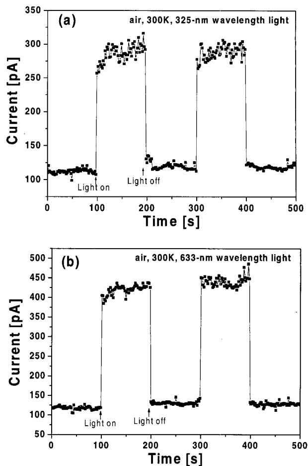
Fig. 4. Time-dependent photocurrents under the illuminations of the 325 nm wavelength light (a) and the 633-nm wavelength light (b).
