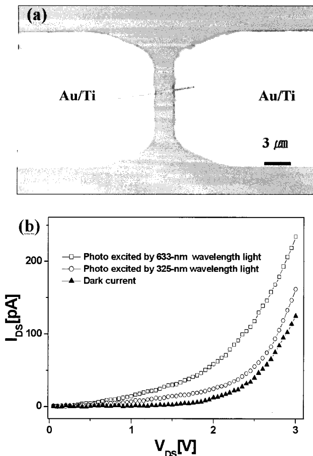
Fig. 3. Optical microscope image (a) of a single-crystalline Si nanowire between two Ti/Au electrodes on a \text{SiO}_2/\text{Si} substrate, and current-voltage ( I - V ) curves (b) for the single-crystalline Si nanowire in the dark and under the illumination of 325-nm and 633-nm wavelength light.
