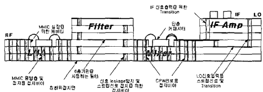
(b) LTCC 수신기 모듈 단면도(A-A') (b) LTCC receiver module cut view(A-A')
