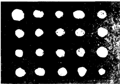
사진 11. Cross-sections of mud pisolites (Ondaigul cave)
