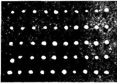
사진 1. Oolites which are initial forms of pisolites (D: 2~3mm, Gosugul cave)
