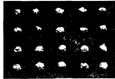
사진 8. Typical pisolites (D: about 1cm, Gosugul cave)
