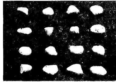
사진 2. Cave pearls which are highly corroded and gloss(Sujeonggul cave and Chodanggul cave)
