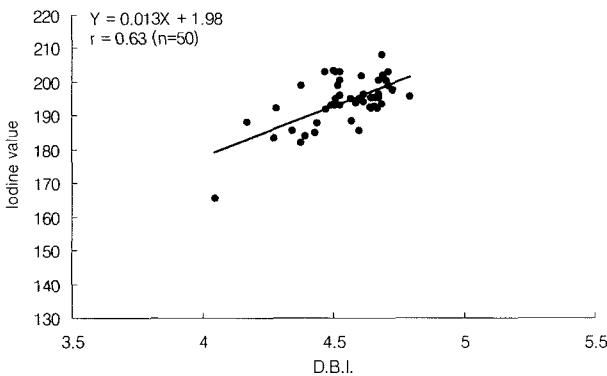
Fig. 1. Relationship between D.B.I. and Iodine value.
