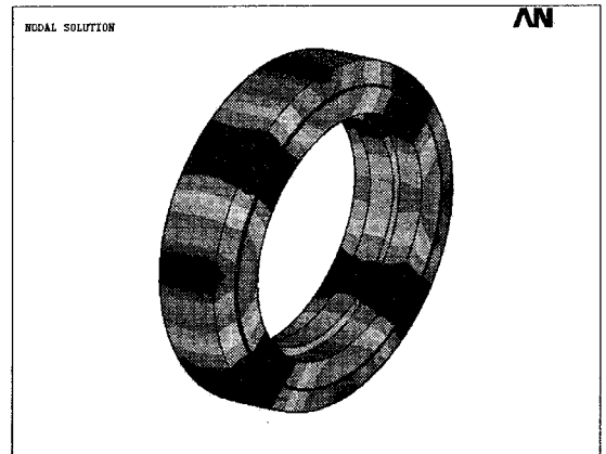
Fig. 13 Result of modal analysis for a urethane wheel : 1 st natural frequency -1925Hz
