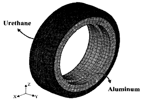
Fig. 2 Finite element model of a urethane wheel
