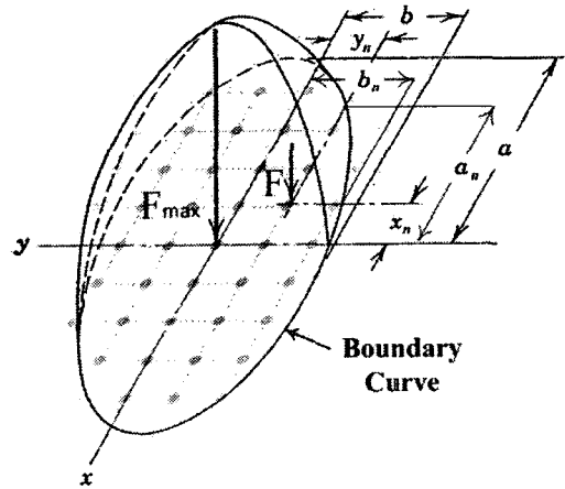
Fig. 5 Ellipsoidal surface force distribution of point Contact
