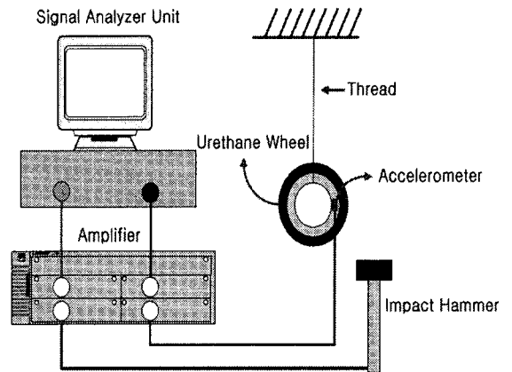
Fig. 14 Vibration test set of a urethane wheel
