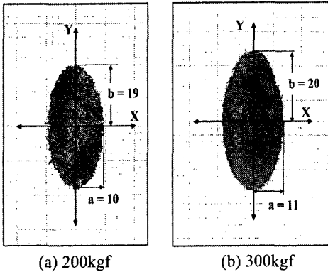
Fig. 4 Results of contact patch test
