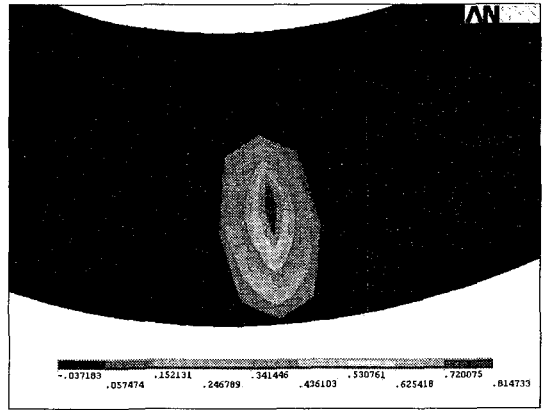
Fig. 10 Maximum displacement of a urethane wheel for 300kgf : 0.81mm
