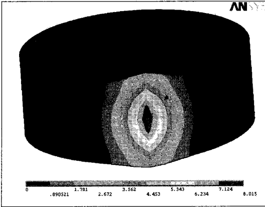
Fig. 12 Maximum stress of an aluminum wheel for 500kgf : 8.0MPa
