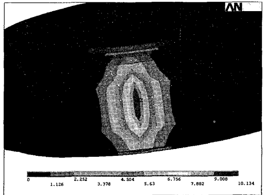
Fig. 11 Maximum stress of a urethane wheel for 500Kgf : 10.1MPa
