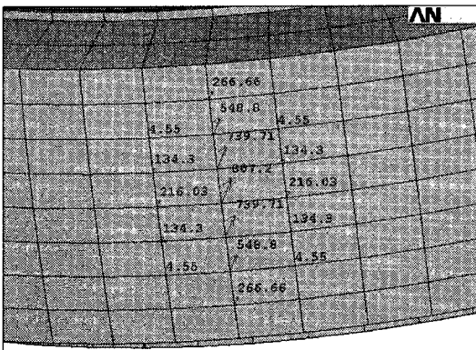
Fig. 7 Force distribution of a urethane wheel for 500kgf
