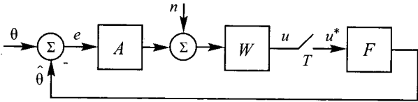
Fig. 1. The sampled PLL linear approximated feedback system.
