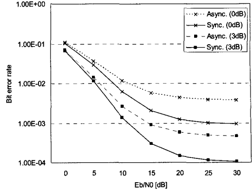
Fig. 1. Uncoded BER vs. Eb/N0 in multiple cells ( K=24 , a^2/\Omega_0=0 or 3dB, \delta=0.2 )
