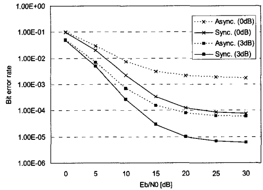
Fig. 2. Uncoded BER vs. Eb/N0 in multiple cells ( K=24 , a^2/\Omega_0=0 or 3dB, \delta=1.0 )
