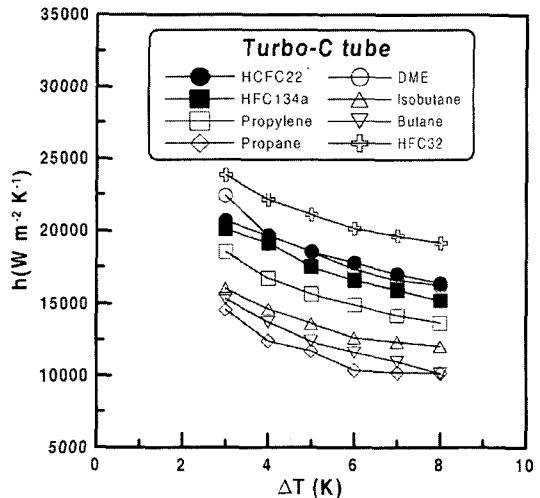
Fig. 3 Condensation HTC's of flammable refrigerants on Turbo-C tube
