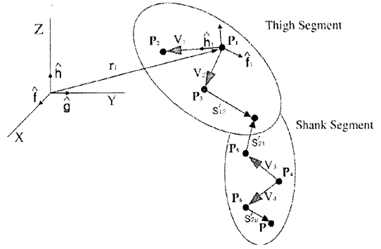
Fig. 4 PBM configuration
