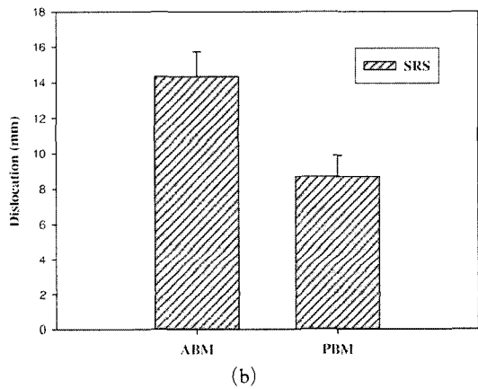
Fig. 8 Joint dislocation at knee for the ABM and PBM based on the LRS (a) and SRS (b)
