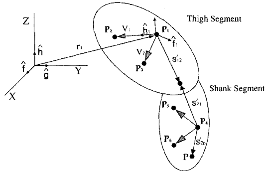
Fig. 3 ABM configuration
