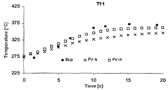
Fig. 11 Comparison with experimental (Exp) and numerical data using the finite volume method with Newtonian boundary conditions (FV-h) and with diffusive boundary conditions (FV-k) for thermocouple T11
