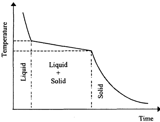
Fig. 1 Metallic alloy cooling curve
