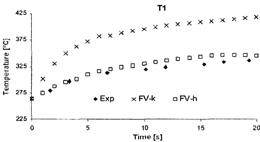
Fig. 9 Comparison with experimental (Exp) and numerical data using the finite volume method with Newtonian boundary conditions (FV-h) and with diffusive boundary conditions (FV-k) for thermocouple T1
