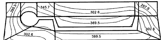
Fig. 7 Mould temperature field at the end of solidification (14,8 seconds of cooling) considering Newtonian heat transfer at interface part/mould
