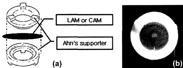
Fig. 2. Ahn's AM supporter. Schematic diagrams of the Ahn's AM supporter (a) and photograph of LAM supported by the Ahn's supporter (b).
