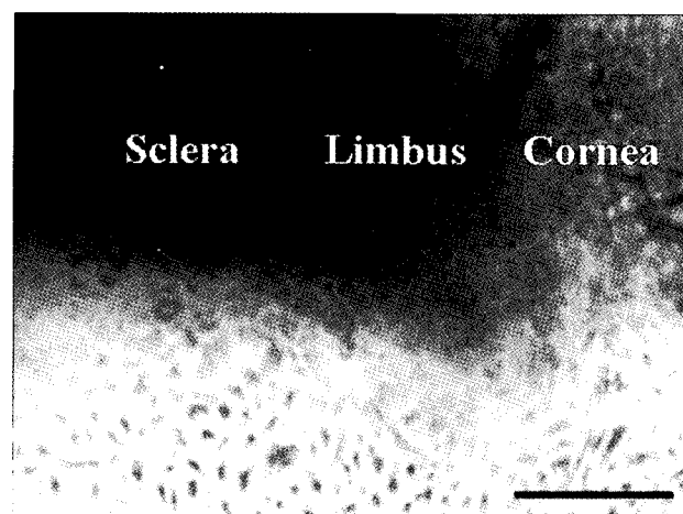
Fig. 1. Primary rabbit corneal epithelial cells from the limbal explantation culture. The upper left part is the sclera, the upper right part the cornea and the lower part the outgrown rabbit corneal epithelial cells. (Bar = 200 \mu\text{m} )
