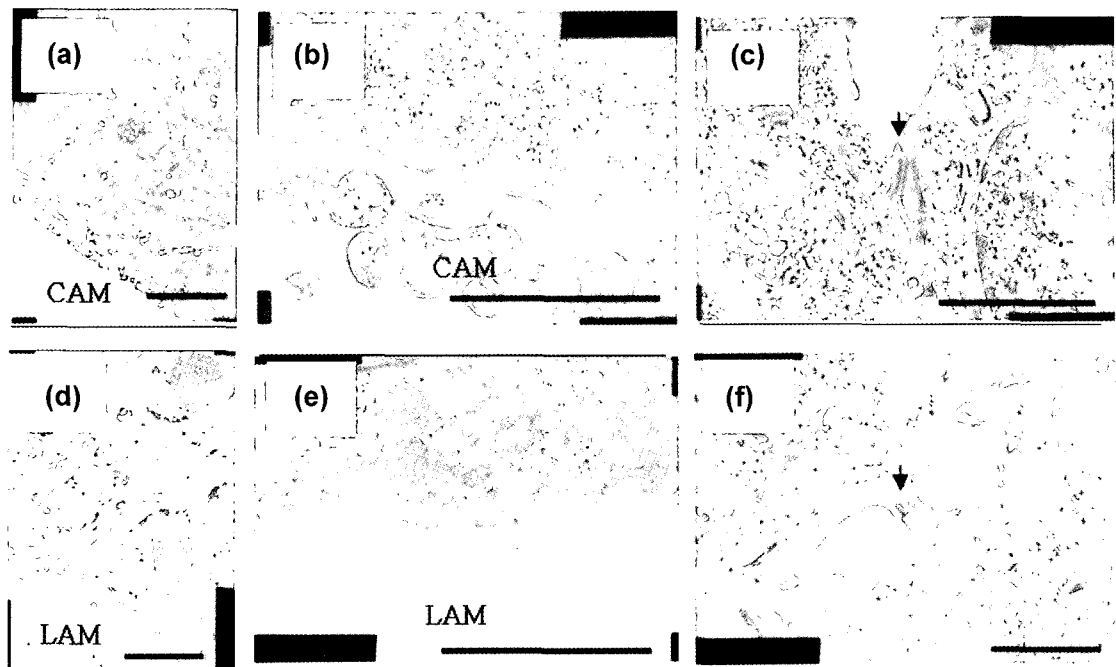
Fig. 8. TEM of the reconstructed bioartificial corneal epithelium on the AM. The basal cells of the reconstructed corneal epithelium on the CAM ((a), Bar = 5 \mu\text{m} ) and LAM ((d), Bar = 5 \mu\text{m} ). Hemidesmosomal cell-cell contacts (arrow) in the corneal epithelium reconstructed on both the CAM ((b), Bar = 1 \mu\text{m} ) and the LAM ((e), Bar = 1 \mu\text{m} ), and the desmosomal cell-cell contact (arrow head) in the corneal epithelium reconstructed on both the CAM ((c), Bar = 1 \mu\text{m} ) and the LAM ((f), Bar = 1 \mu\text{m} ).
