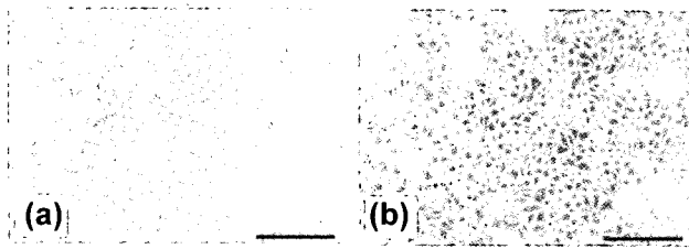
Fig. 4. Photograph of corneal epithelial cells at third passage on plastic dish (a) and the inoculated third passage corneal epithelial cells on LAM (b). (Bar = 200 \mu m)
