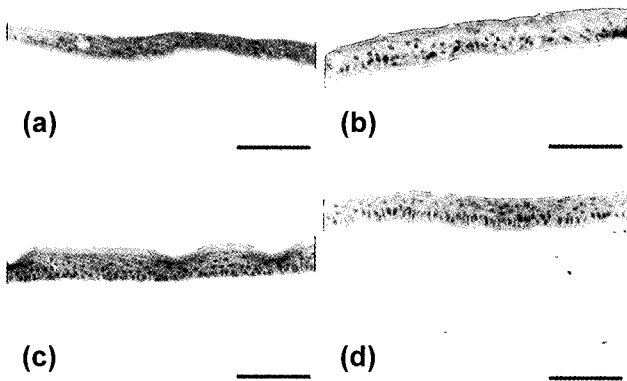
Fig. 5. Histology of the reconstructed bioartificial corneal epithelium on the AM (Hematoxylin & eosin staining). The reconstructed corneal epithelium on the LAM for 3 days (a), the reconstructed corneal epithelium on the LAM (b) and CAM (c) for 6 days, normal rabbit corneal epithelium (d). (Bar = 100 \mu m)
