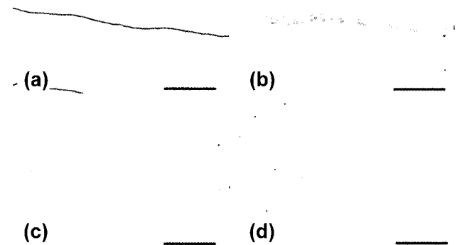
Fig. 7. Immunohistology of the reconstructed bioartificial corneal epithelium on the AM (p63 staining). The reconstructed corneal epithelium on the LAM for 3 days (a), the reconstructed corneal epithelium on the LAM (b) and CAM (c) for 6 days, normal rabbit corneal epithelium (d). (Bar = 100 \mu m)
