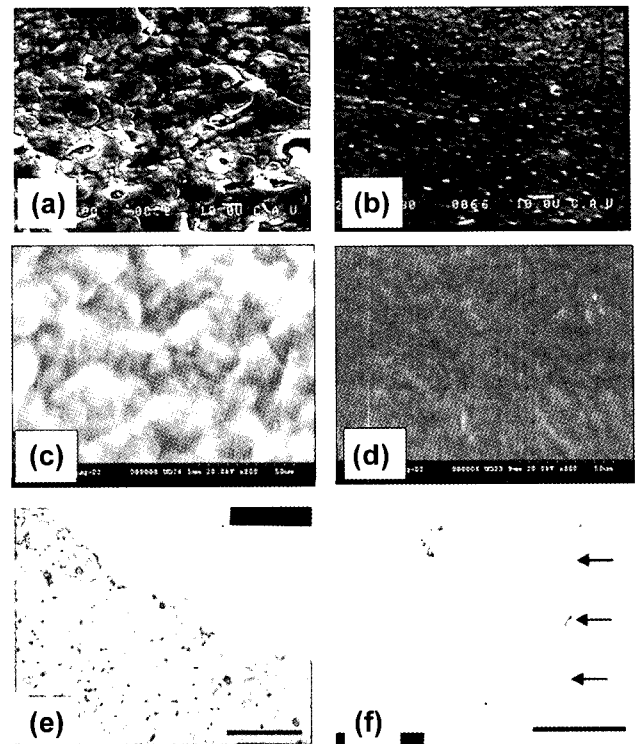
Fig. 3. Preparation of the AM. SEM images of CAM and LAM before (a, c) and after removal of amniotic epithelial cells (b, d). TEM images of AM before ((e), bar = 10 μm) and after ((f), Bar = 5 μm) removal of amniotic epithelial cells.
