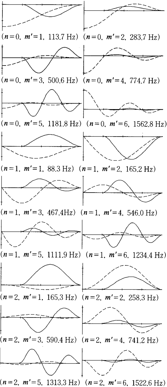
Fig. 3 Theoretical mode shapes of an annular plate and a circular plate coupled with water (solid line=upper annular plate, dashed line= lower circular plate)
