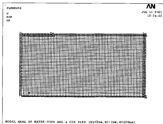
Fig. 2 Finite element model for the fluid contained vessel with an annular plate and a circular plate
