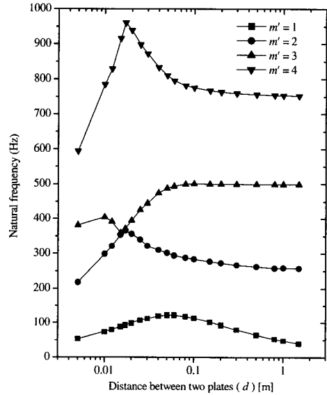
Fig. 4 Natural frequency vs. distance between the plates for n=0
