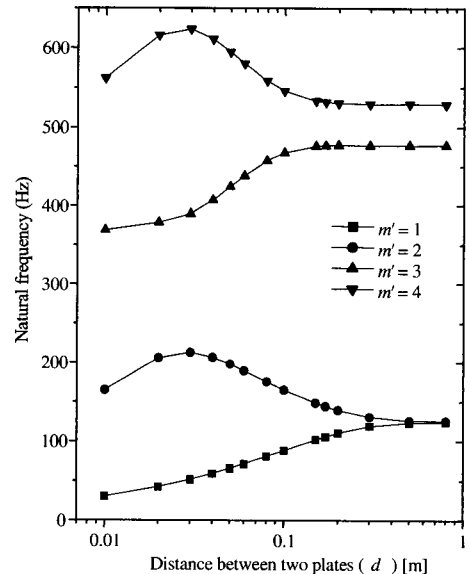
Fig. 5 Natural frequency vs. distance between the plates for n=1
