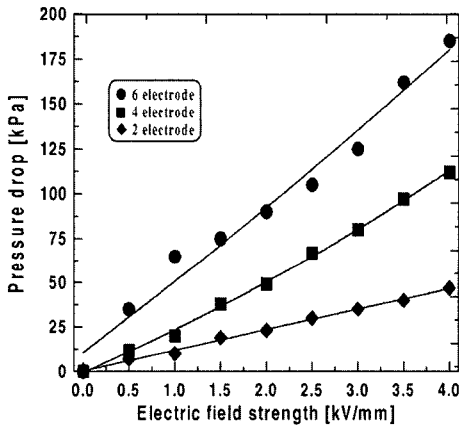
Fig. 5 Pressure drop and electric field strength of ER Valve
