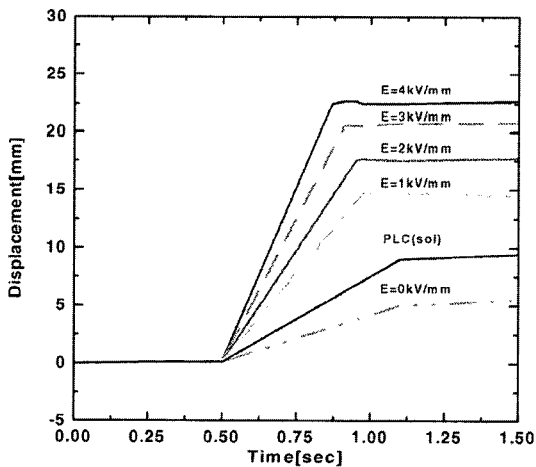
(b) 2 Electrodes
