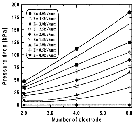
Fig. 6 Pressure drop and number of electrode of ER Valve
