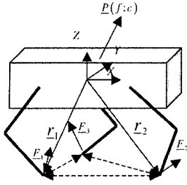
Fig. 15 Three-legged system
