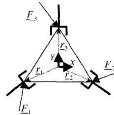
Fig. 5 Triple manipulator in planar domain
