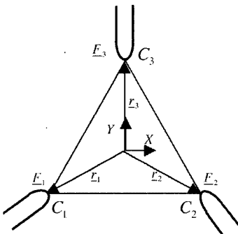
Fig. 14 Three-fingered system
