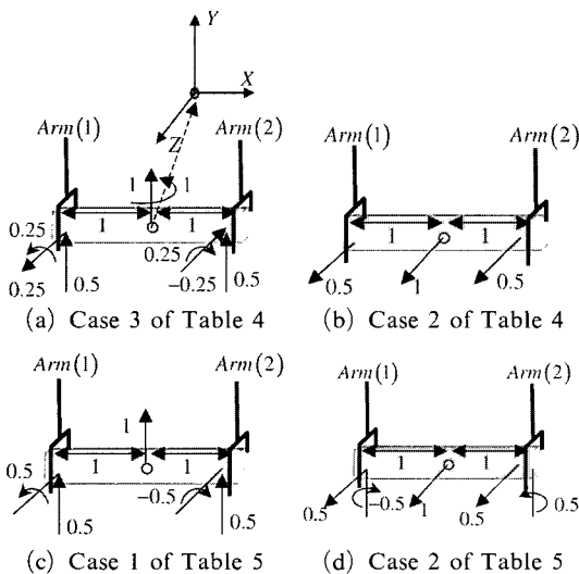
Fig. 12 Comparison of internal loadings for two cases
