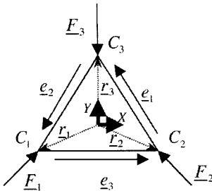
Fig. 13 Internal force
