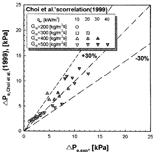
Fig. 6 Comparison of the measured pressure drop data with those predicted by Choi et al.'s correlation.
