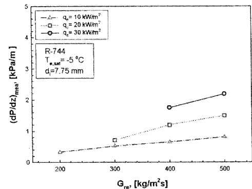
(b) T_{e,sat} = -5^\circ C
