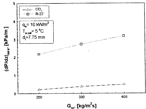
Fig. 5 Comparison of the pressure drop of CO 2 and R-22 at saturation temperature of 5°C and heat flux of 10 kW/m 2 .
