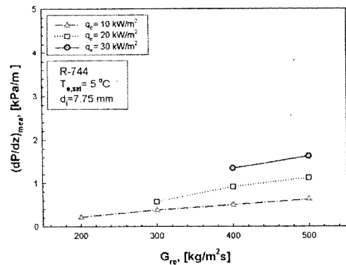
(a) T_{e,sat} = 5^\circ C
