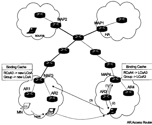
Figure 1. M-HMIPv6 handover
