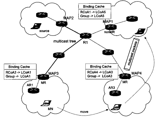
Figure 2. HMMIPv6 scheme
