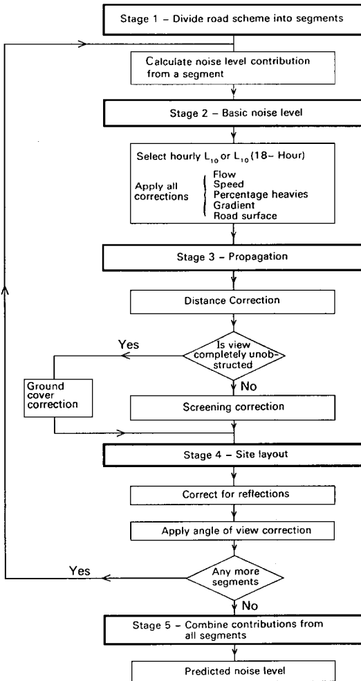
Fig. 1 Flow chart for predicting noise from road schemes (2)
