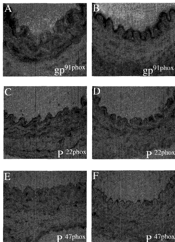
Fig. 5. Photomicrographs ( \times 400 ) showing expression of gp91phox, p22phox and p47phox in frozen sections of aorta from control (A through C) and ob/ob mice (D through F). The location of each antigen was indicated by the dark brown reaction product generated by DAB system. The nuclei were counterstained with Mayer's hematoxylin.
