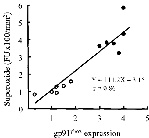
Fig. 6. Superoxide production was plotted as a function of endothelial expression of gp91phox in the aorta from control (open circle) and ob/ob mice (filled circle). FU represents fluorescence unit.
