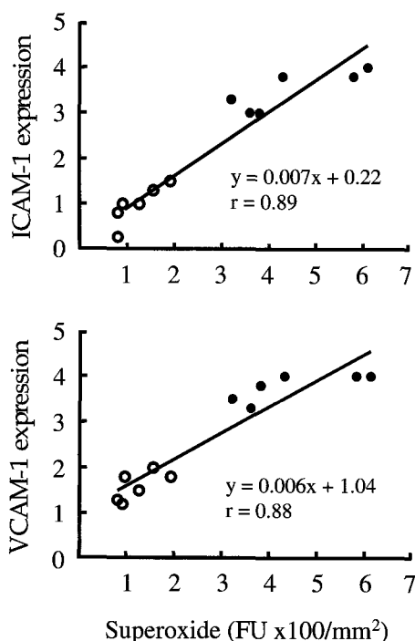
Fig. 4. Endothelial expression of ICAM-1/VCAM-1 was plotted as a function of superoxide production in the aorta from control (open circle) and ob/ob mice (filled circle). FU represents fluorescence unit.
