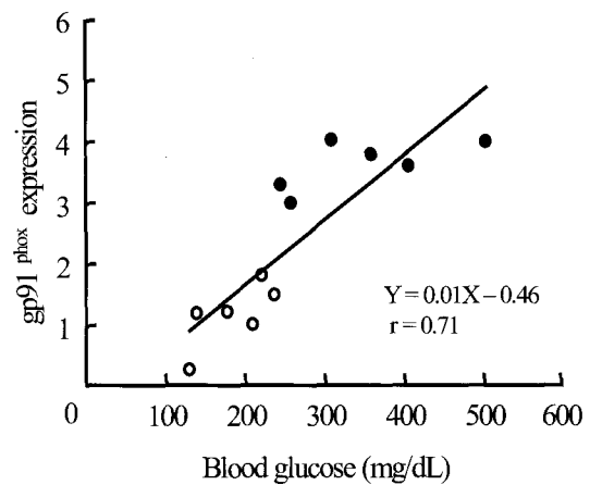
Fig. 7. Endothelial expression of gp91phox was plotted as a function of levels of blood glucose from control (open circle) and ob/ob mice (filled circle).
