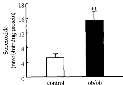
Fig. 2. Superoxide generation from aortic homogenates was determined by lucigenin-enhanced chemiluminescence in response to NADH/NADPH ( 100 \mu\text{M} ) as potential substrates. Bars represent mean±SEM from 5 experiments. **P<0.01 vs. control.
