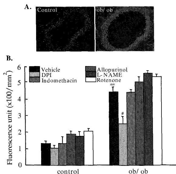
Fig. 1. (A) Representative photographs ( \times 200 ) of dihydroethidium-stained aortic sections from control and ob/ob mice. The intensity of red fluorescence in sections represents the amount of superoxide generated. (B) Effects of various inhibitors such as DPI ( 10 \mu\text{M} ), indomethacin ( 10 \mu\text{M} ), allopurinol ( 100 \mu\text{M} ), L-NAME ( 100 \mu\text{M} ), and rotenone ( 100 \mu\text{M} ) on superoxide production in control and diabetic aorta. Data are presented as means±SEM from 6 experiments in each group. **P<0.01 vs. corresponding value in control. # P<0.05 vs. corresponding vehicle.
