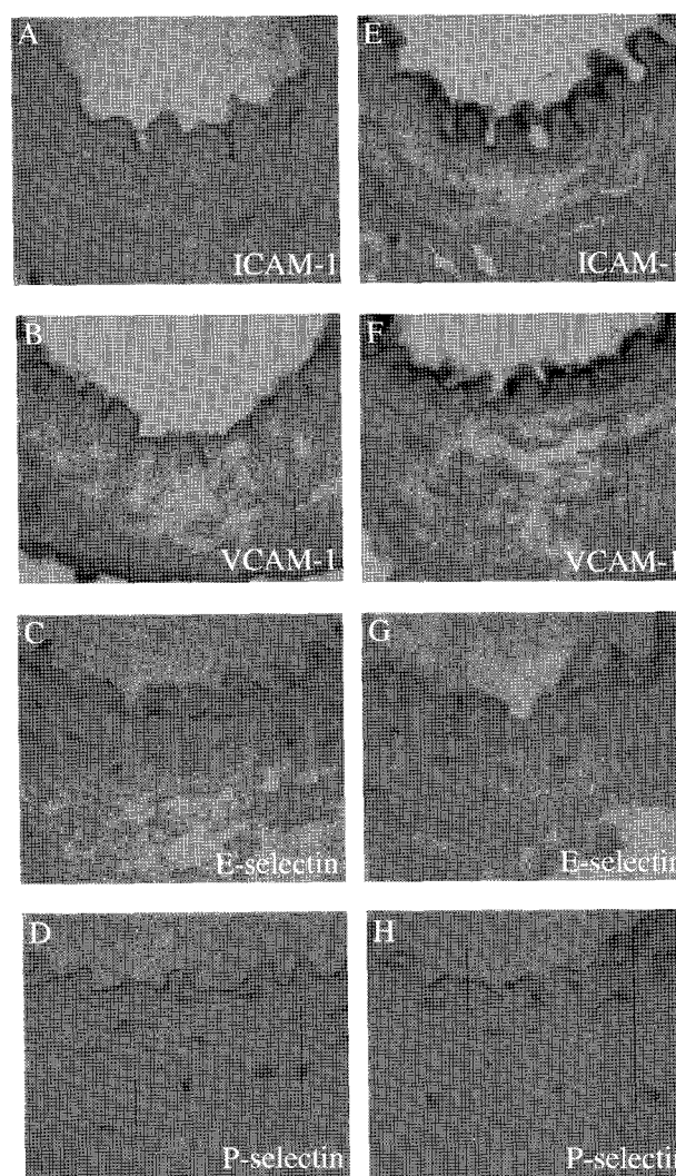
Fig. 3. Photomicrographs ( \times 400 ) showing expression of ICAM-1, VCAM-1, E- and P-selectin in frozen sections of aorta from control (A through D) and ob/ob mice (E through H). The location of each antigen was indicated by the dark brown reaction product generated by DAB system. The nuclei were counterstained with Mayer's hematoxylin.
