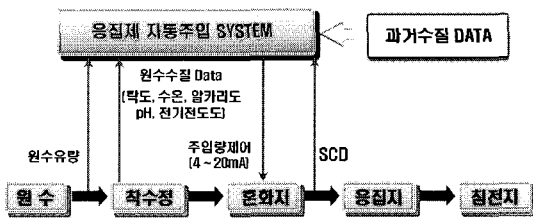
Fig. 3 Block diagram of coagulation dosing process
