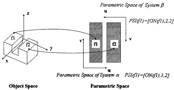
Fig. 7. Difference in PSI (parametric space information) among CAD systems [15].
