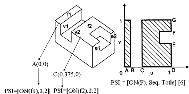
Fig. 4-3. Ambiguity solving based on geometric information [6] ( Problem 1.1.2 ).
