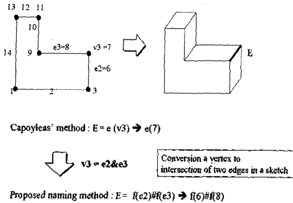
Fig. 13. Mapping of basic name.
