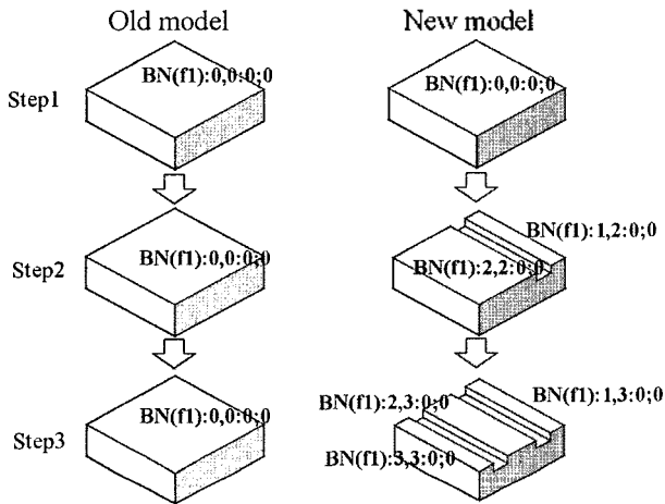
Fig. 10. Name matching problem arising from face splitting [15].
