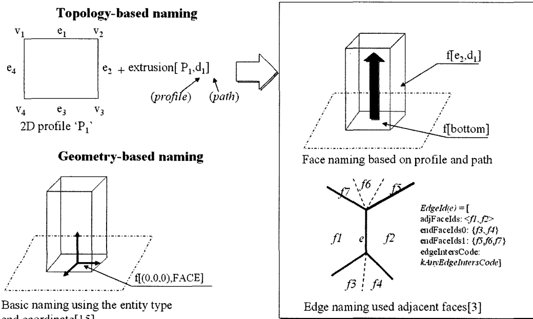
Fig. 3. Basic naming (Problem 1.1.1).
