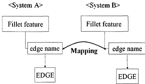
Fig. 2-3. Naming mapping problem.
