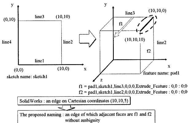
Fig. 16. Naming mapping between SolidWorks and the proposed naming.
