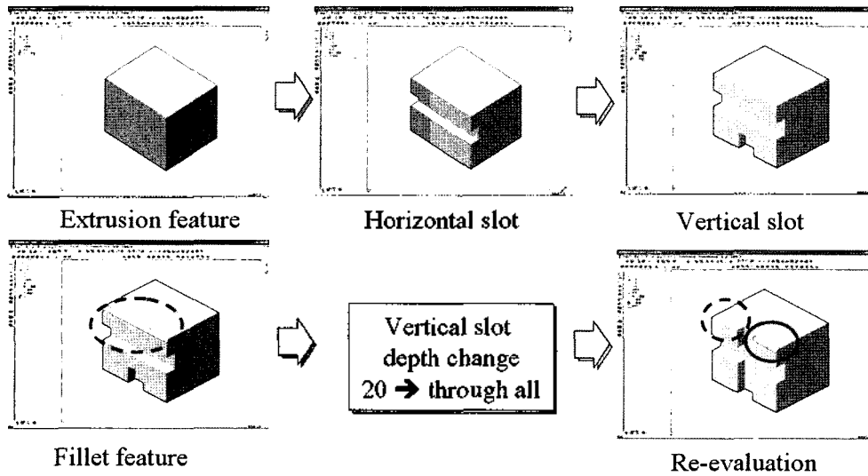
Fig. 1. A persistent naming problem in SolidWorks.
