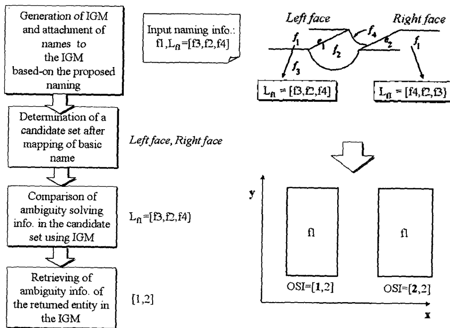
Fig. 14. Mapping ambiguity solving information.
