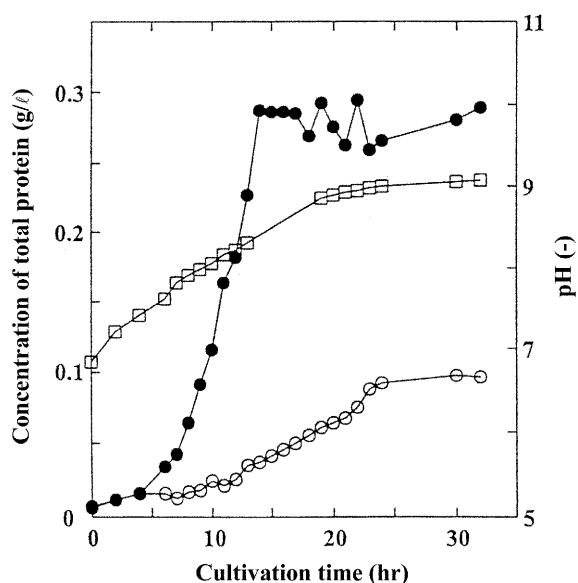
Figure 1. Effects of purging with N_2 on growth of Desulfovibrio vulgaris Miyazaki F. The open and closed circles represent non-purging and purging with N_2 , respectively. The open squares represent the pH of culture under purging with N.
