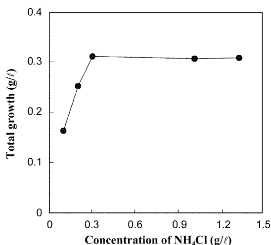
Figure 3. Effects of ammonium chloride concentration on total growth in defined medium.
