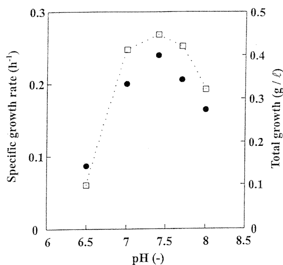
Figure 2. Influence of pH on a specific growth rate and total growth. The closed circles represent the specific growth rate. The open squares represent the total growth. Full line show model fitting from the equation, \mu = \mu_{\max} / (1 + H^+/K_H + K_{OH}/H^+) Where K_H and K_{OH} are rate constants.
