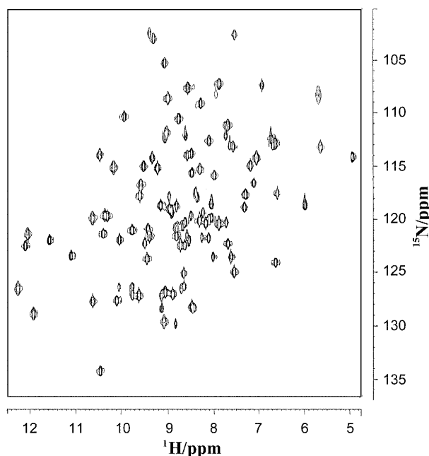
Figure 4. Section of a ^1\text{H} - ^{15}\text{N} HMQC spectrum of ferricytochrome c_3 . The spectrum was acquired at 30 °C, pH 5.0, in \text{H}_2\text{O} . The spectrum was acquired with spectral widths of 4000 Hz for ^1\text{H} and 5000 Hz for ^{15}\text{N} , 4 K data points in t_2 , and 32 transients for each of 512 t_1 points. ^1\text{H} chemical shifts were referenced to the ^1\text{H}_2\text{O} signal at 4.73 ppm. ^{15}\text{N} chemical shifts were referenced to external saturated \text{NH}_4\text{Cl} at 27.34 ppm.
