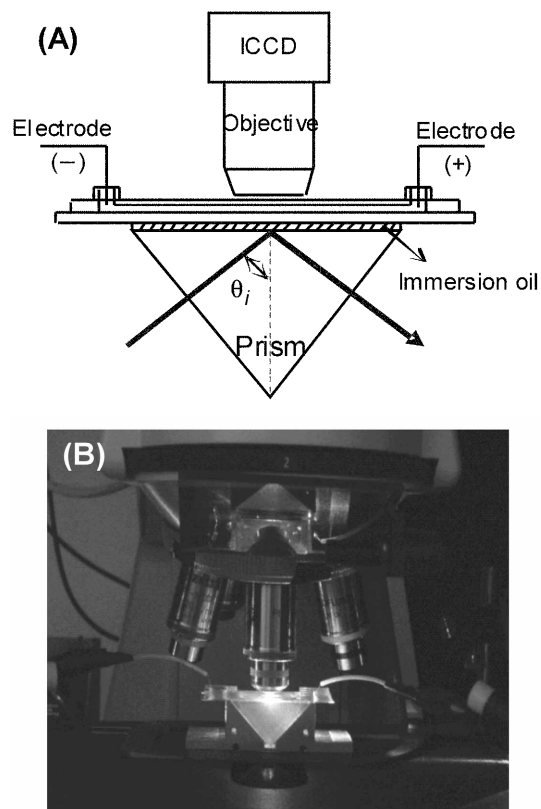
Figure 1. (A) Schematic diagram and (B) picture of TIRFM experiment setup at the PDMS/glass microfluidic chip for single-DNA molecule monitoring within the evanescent field layer.
