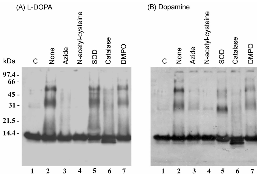
Figure 3. Effect of radical scavengers on the aggregation of \alpha -synuclein by oxidized catechols. \alpha -Synuclein (0.25 mg/ml) was incubated with 30 \mu\text{M} L-DOPA (A) or 30 \mu\text{M} dopamine (B) at 37 ^{\circ}\text{C} for 12 h in the presence of radical scavengers. Lane 1, \alpha -synuclein control; lane 2, no addition of effectors; lane 3, 200 mM azide; lane 4, 50 mM N-acetyl cysteine; lane 5, SOD (0.2 mg/mL); lane 6, catalase (0.1 mg/ml); lane 7, 10 mM DMPO. The samples were analyzed by immunoblotting.
