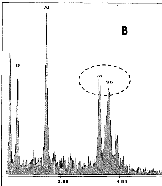
Fig. 3. EDS results measured from the "A" and "B" part in Fig. 2.
