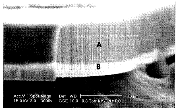
Fig. 2. A SEM image of AAO nano-template filled partly with InSb nanowires.
