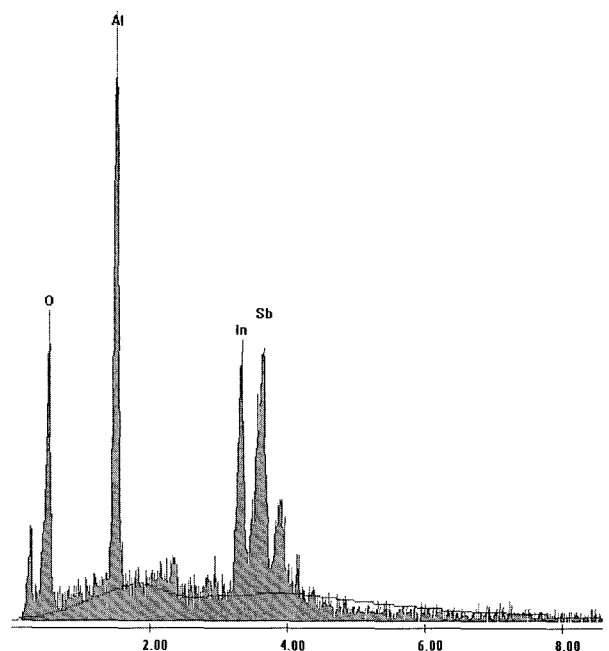
Fig. 5. An EDS result of the InSb nanowires in Fig. 4.
