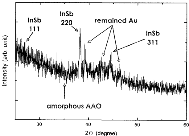
Fig. 7. X-ray diffraction patterns measured at the InSb nanowires of Fig. 6.
