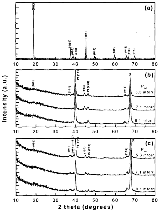
Fig. 3. X-ray diffraction patterns of : (a) LiCoO 2 target, (b) as-deposited, and (c) annealed at 400°C for 5 hours.
