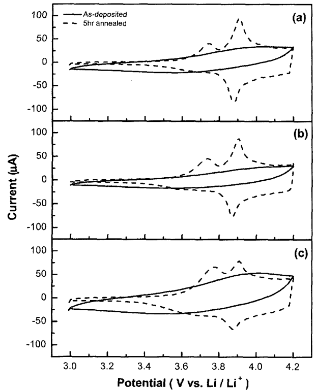
Fig. 1. Cyclic voltammograms of as-deposited and annealed half cell as a function of the P Ar for LiCoO 2 deposition. (a) P Ar = 9.1, (b) P Ar = 7.1, and (c) P Ar = 5.3 mTorr.
