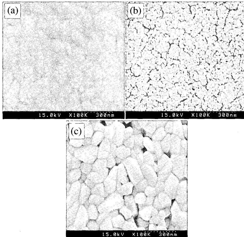
Fig. 4. SEM images of annealed LiCoO 2 thin films deposited at 9.1 mTorr (a) as-deposited, (b) annealed at 400°C, and (c) 700°C for 1hr.
