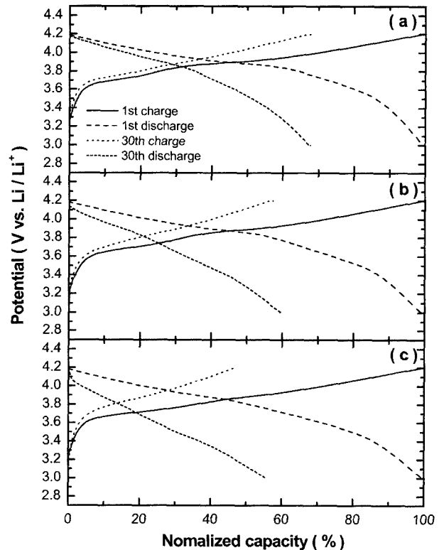
Fig. 2. Charge-discharge curves of half cells composed of liquid electrolyte with as-deposited and annealed LiCoO 2 thin films deposited at (a) P Ar = 9.1, (b) P Ar = 7.1 and (c) P Ar = 5.3 mTorr, respectively.
