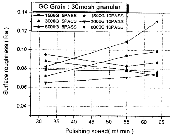
(b) granular structure type magnetic abrasive: GC
