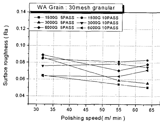
(a) granular structure type magnetic abrasive: WA
