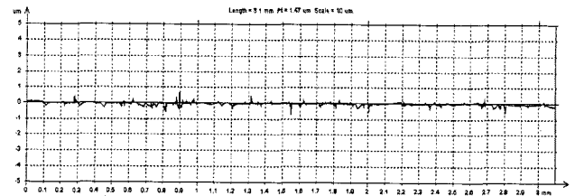
Fig. 5. Surface roughness profile after magnetic polishing(WA, 63.6 m/min, 1500G, 5 Pass).
