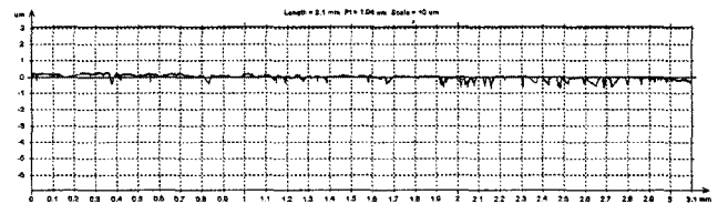
Fig. 3. A surface roughness curve of internal face in STS304 tube.
