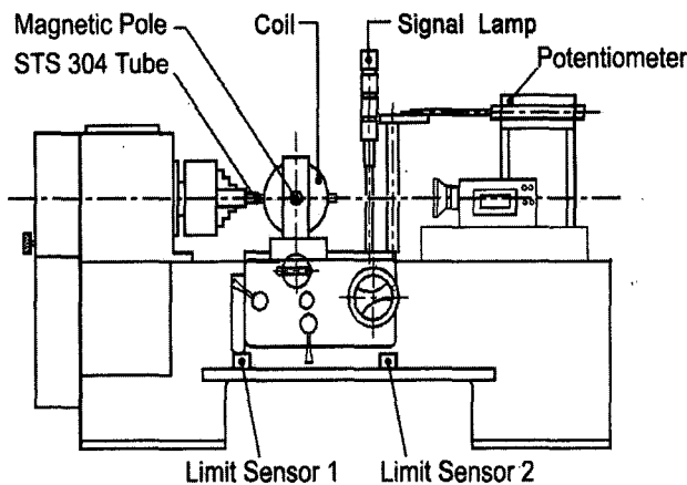
Fig. 1. A schematic of experimental set up.
