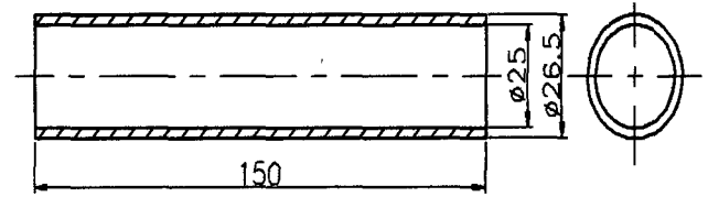
Fig. 2. Geometry and dimension of specimen.
