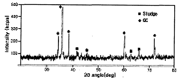
(b) Sludge + GC
