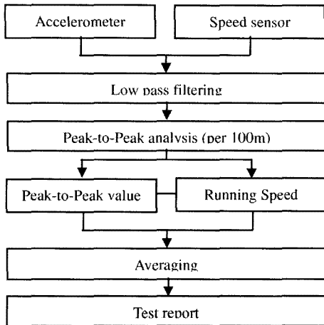
Fig. 5 Procedure of vibration level evaluation
