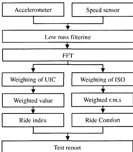
Fig. 3 Procedure of ride comfort evaluation
