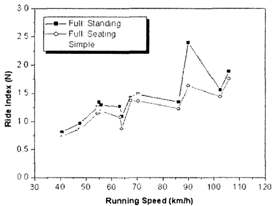
Fig. 8 Ride indices on running speed
