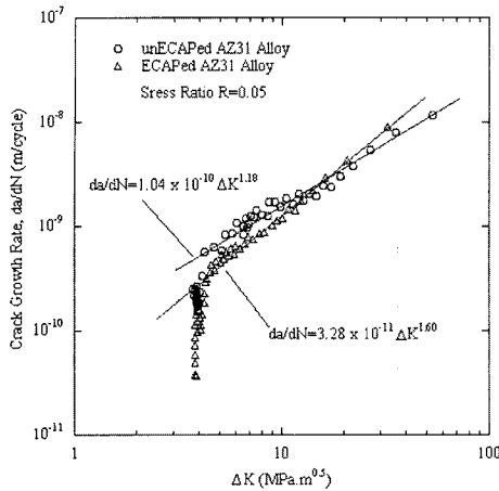
Fig. 6 A comparison of fatigue crack growth behavior of the unECAP and ECAPed AZ31 alloys
