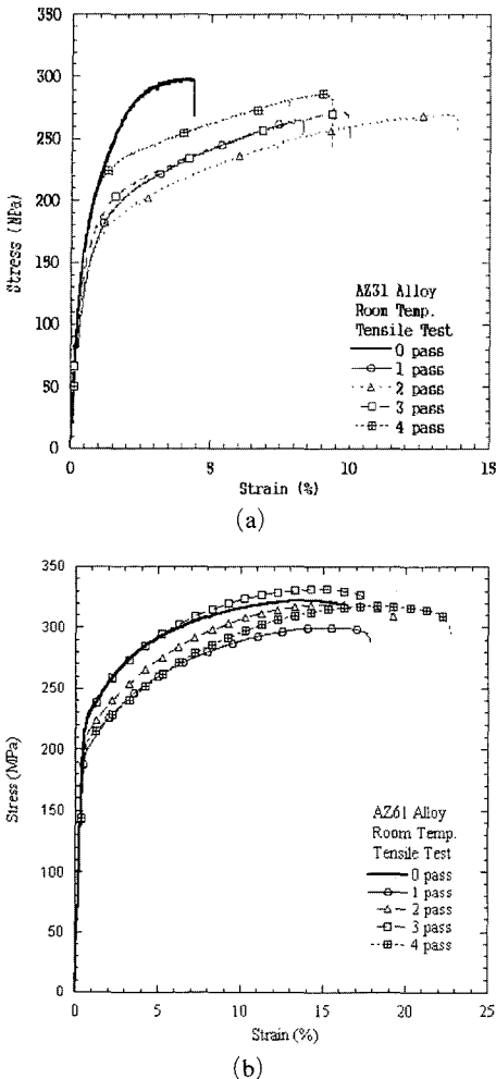
Fig. 4 Stress-strain curves for the unECAP and ECAPed (a) AZ31 and (b) AZ61 alloys
