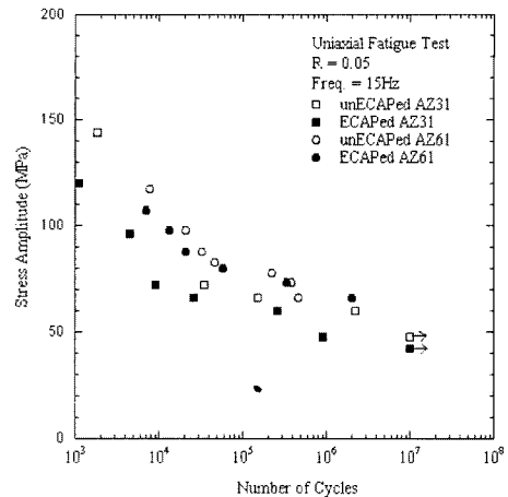
Fig. 5 The S-N curves for the unECAPed and ECAPed AZ31 and AZ61 alloys
